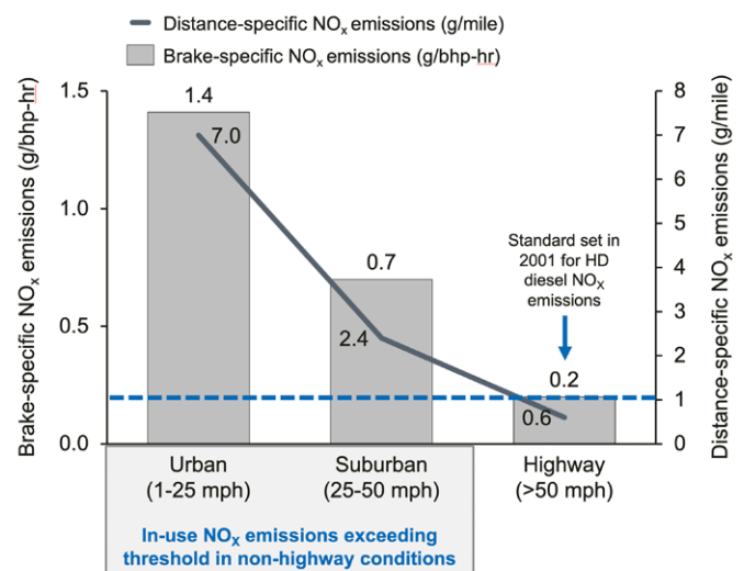
FIGURE 27: AVERAGE IN-USE NO x EMISSIONS FROM MODEL YEAR 2010–2016 HEAVY-DUTY DIESEL VEHICLES
