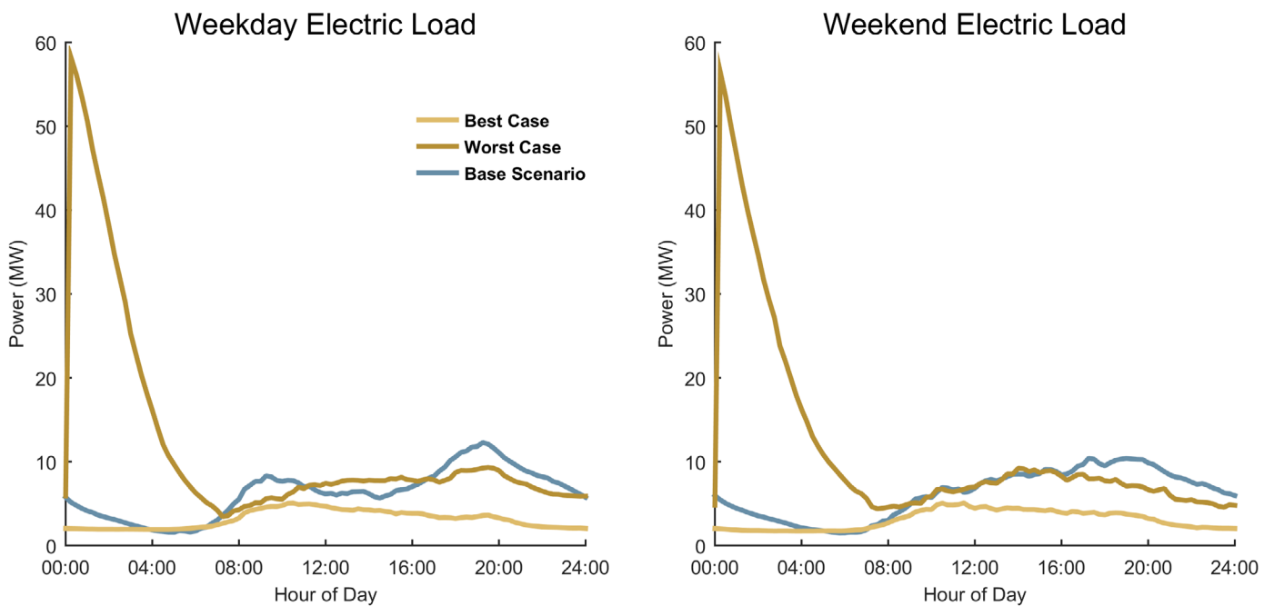
Baseline-, Worst- case, and Best-case load profiles for Aggressive EV adoption for Anchorage urban area
