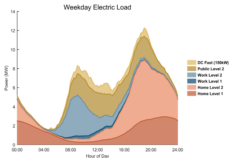
Load Forecasts for Anchorage under an Aggressive Adoption Scenario
