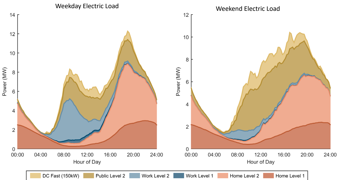
Load Profile for Aggressive EV adoption scenario of Anchorage urban area
