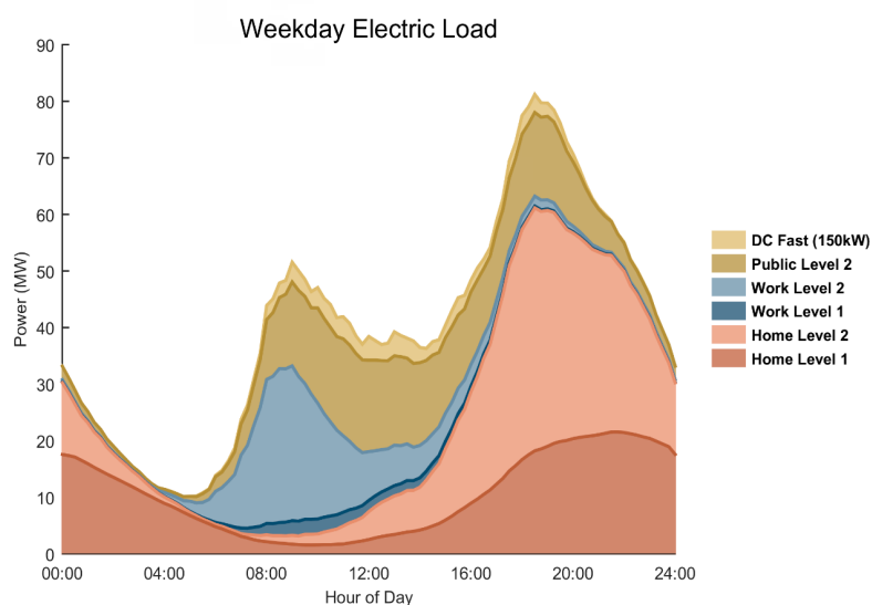
Load Forecasts for Birmingham under an Aggressive Adoption Scenario
