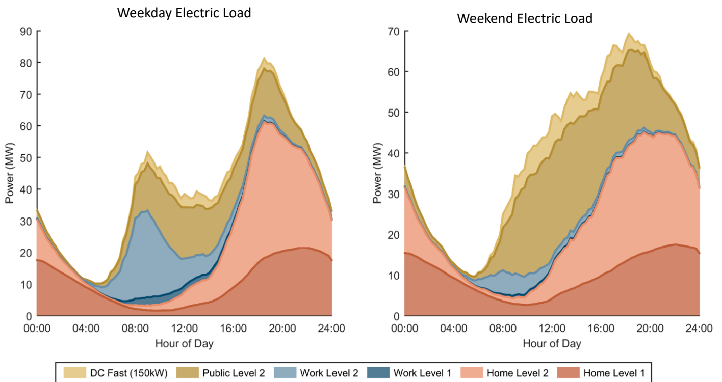
Load Profile for Aggressive EV adoption scenario of Birmingham urban area
