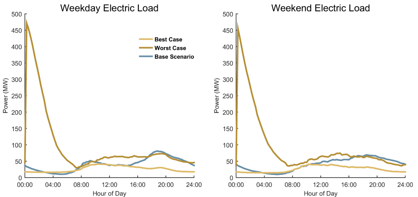
Baseline-, Worst- case, and Best-case load profiles for Aggressive EV adoption for Birmingham urban area
