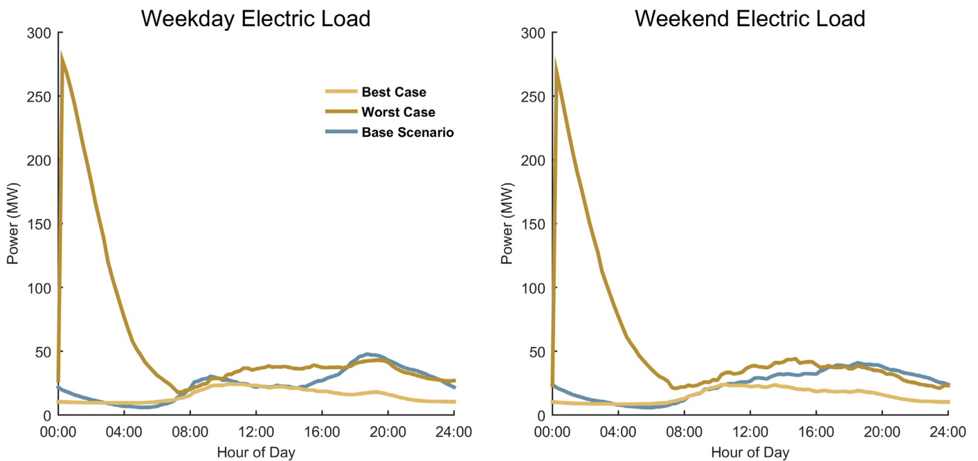
Baseline-, Worst- case, and Best-case load profiles for Aggressive EV adoption for Little Rock urban area
