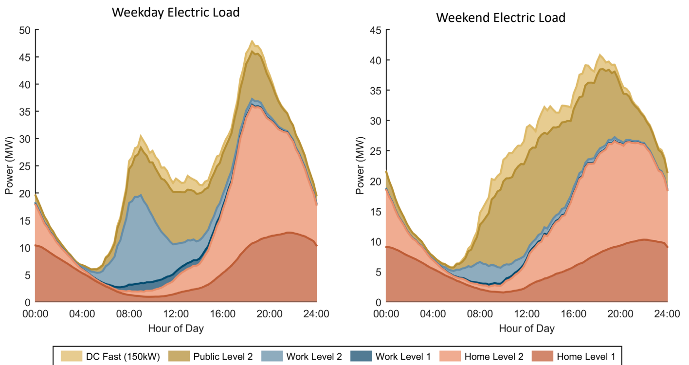
Load Profile for Aggressive EV adoption scenario of Little Rock urban area
