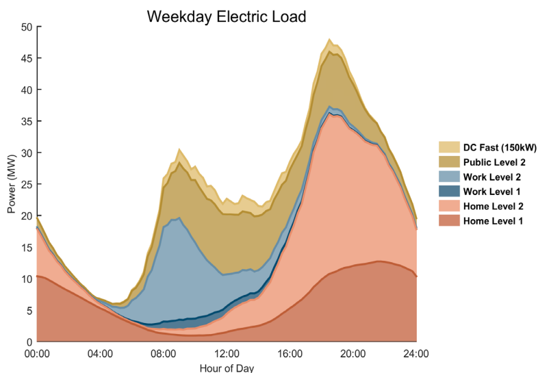
Load Forecasts for Little Rock under an Aggressive Adoption Scenario
