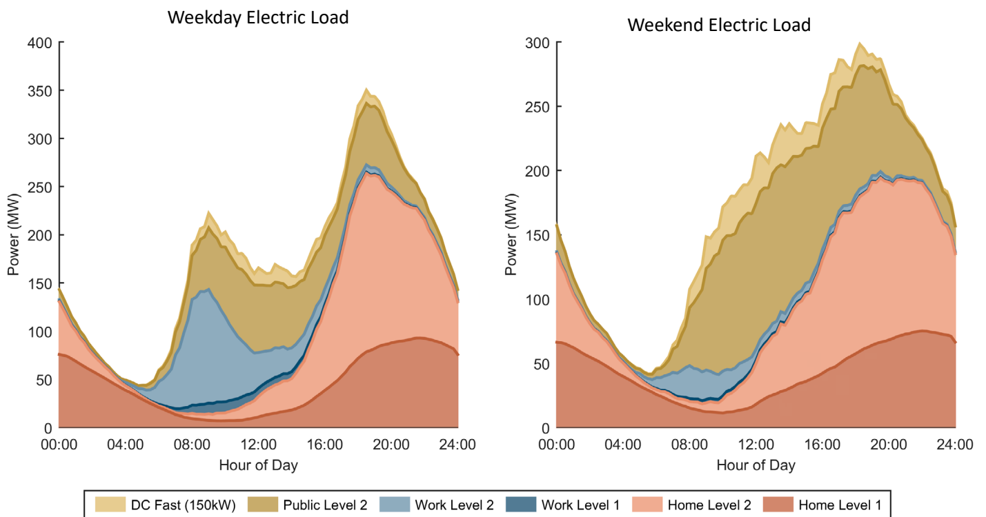
Load Profile for Aggressive EV adoption scenario of Phoenix-Mesa urban area
