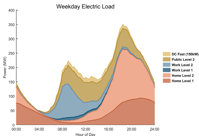
Load Forecasts for Phoenix under an Aggressive Adoption Scenario
