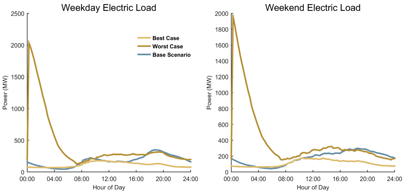
Baseline-, Worst- case, and Best-case load profiles for Aggressive EV adoption for Phoenix-Mesa urban area
