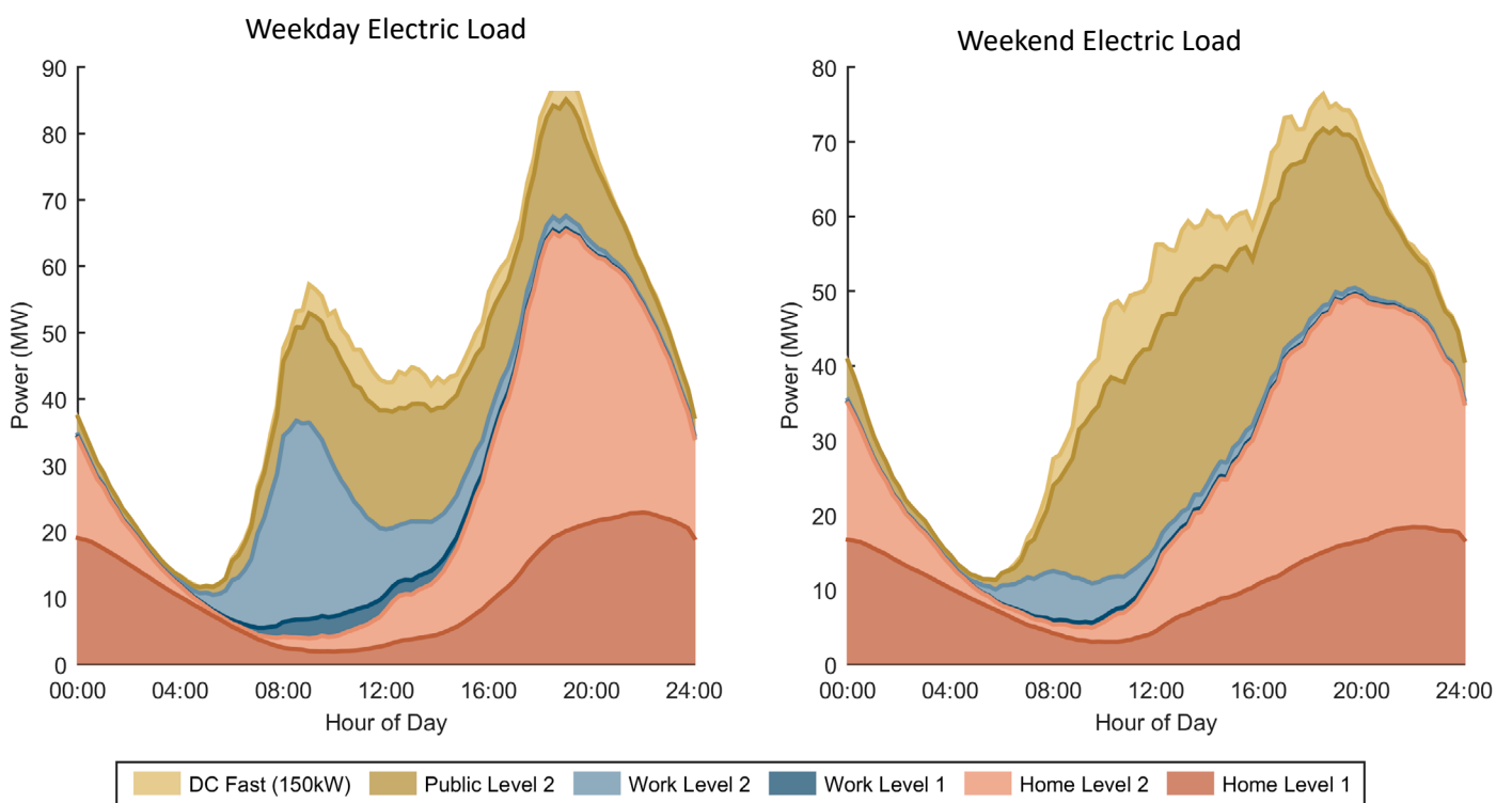
Load Profile for Aggressive EV adoption scenario of Bridgeport - Stamford urban area
