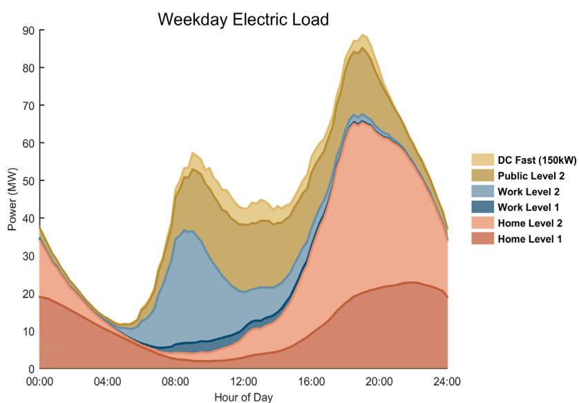
Load Forecasts for Bridgeport under an Aggressive Adoption Scenario
