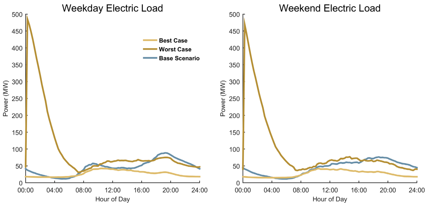
Baseline-, Worst- case, and Best-case load profiles for Aggressive EV adoption for Bridgeport - Stamford urban area
