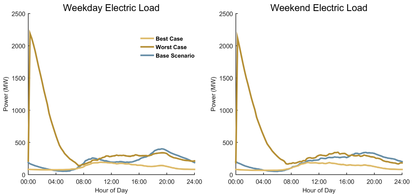
Baseline-, Worst-case, and Best-case load profiles for Aggressive EV adoption for Washington, D.C. urban area
