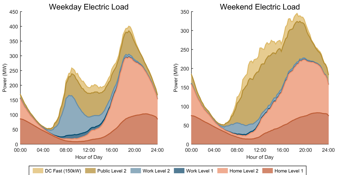
Load Profile for Aggressive EV adoption scenario of Washington, D.C. urban area
