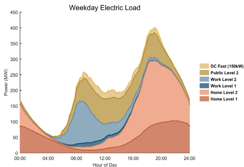
Load Forecasts for Washington, D.C. under an Aggressive Adoption Scenario
