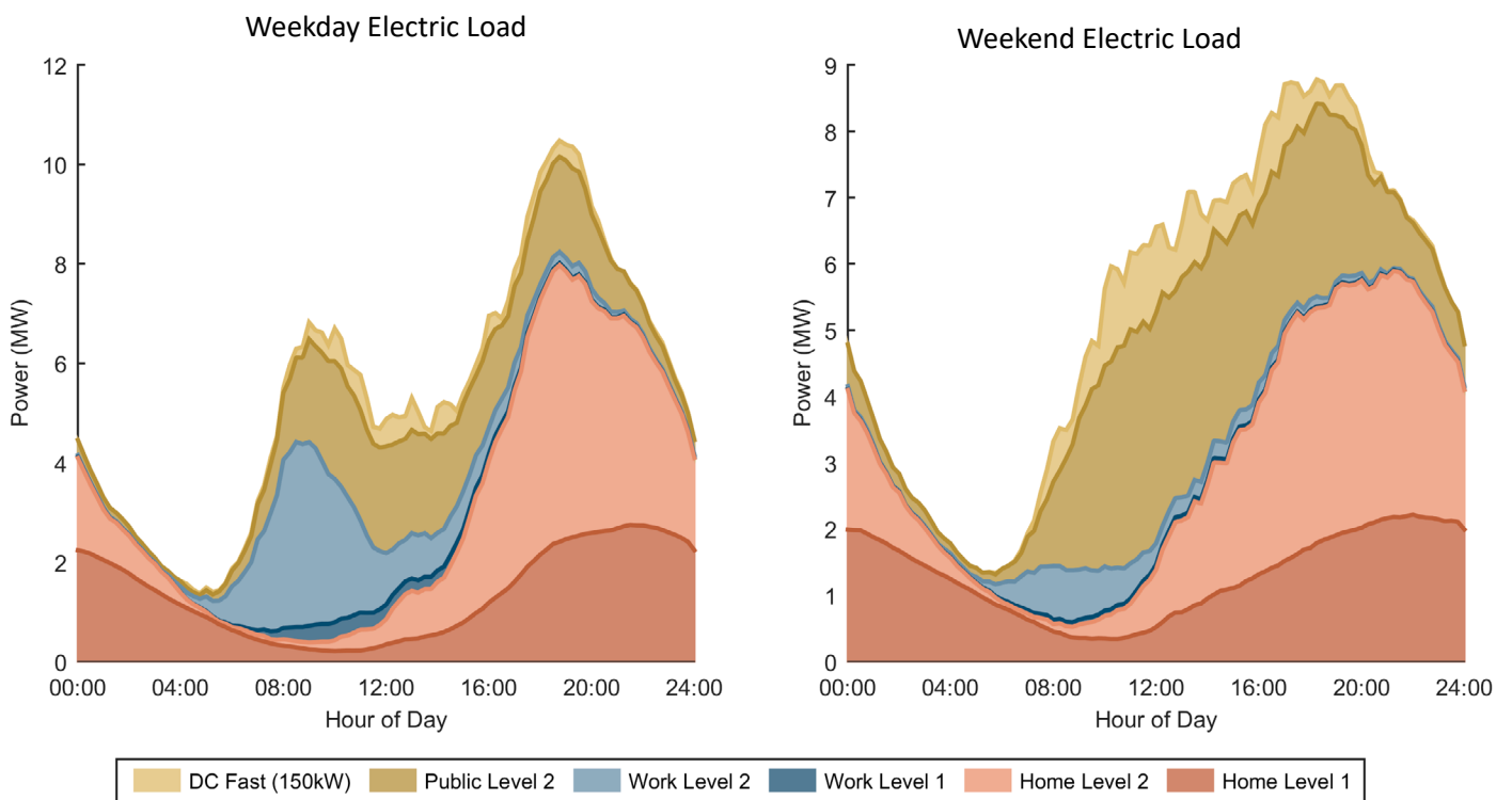
Load Profile for Aggressive EV adoption scenario of Dover urban area
