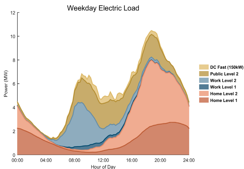
Load Forecasts for Dover under an Aggressive Adoption Scenario
