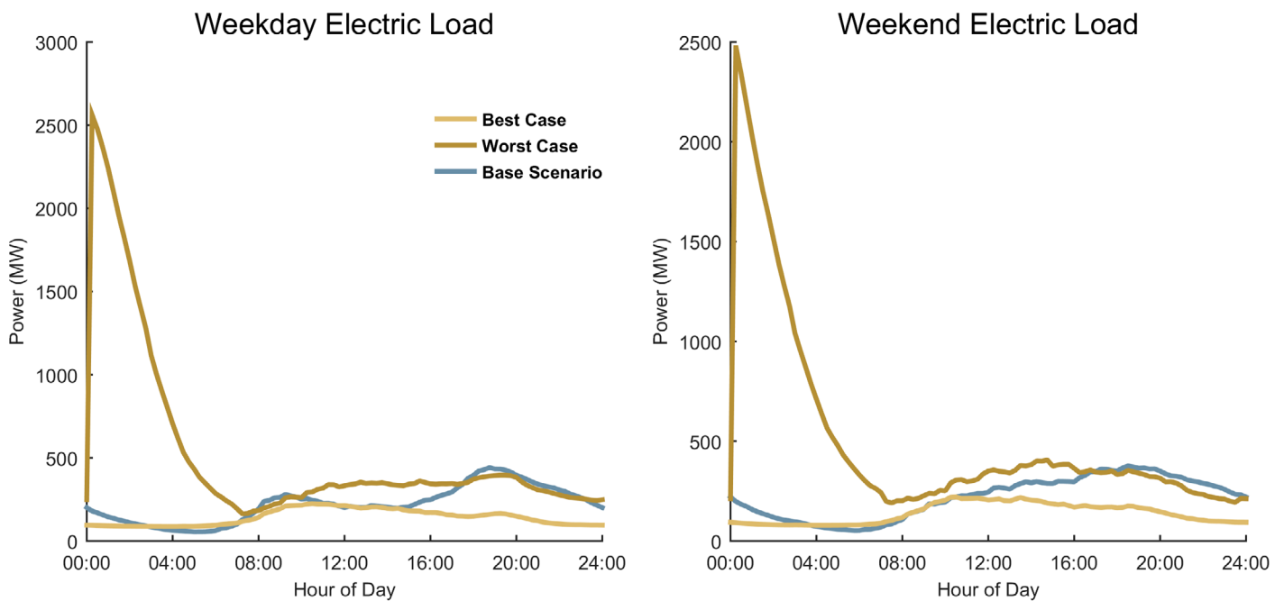
Baseline-, Worst- case, and Best-case load profiles for Aggressive EV adoption for Atlanta urban area
