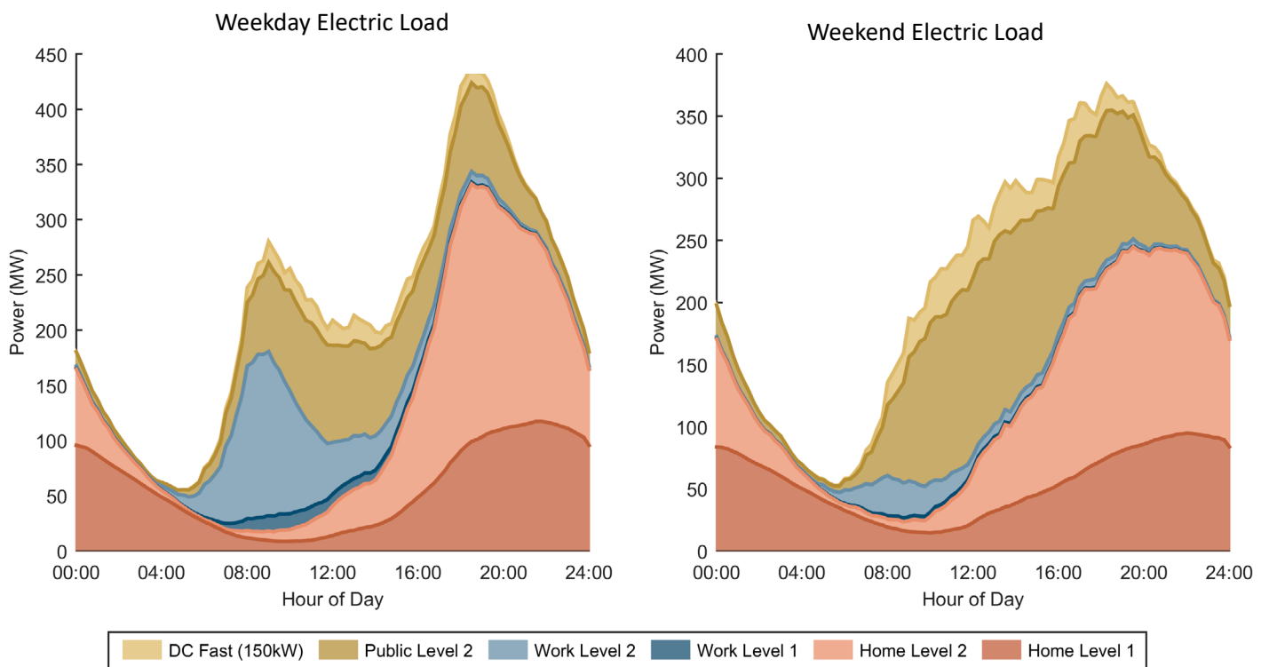
Load Profile for Aggressive EV adoption scenario of Atlanta urban area
