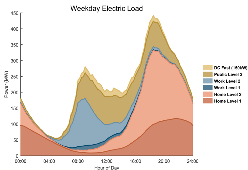
Load Forecasts for Atlanta under an Aggressive Adoption Scenario
