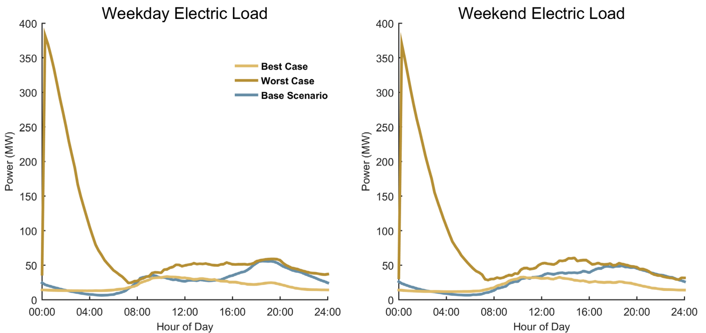
Baseline-, Worst- case, and Best-case load profiles for Aggressive EV adoption for Honolulu urban area
