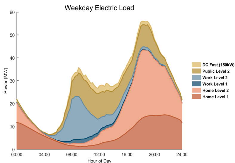
Load Forecasts for Honolulu under an Aggressive Adoption Scenario
