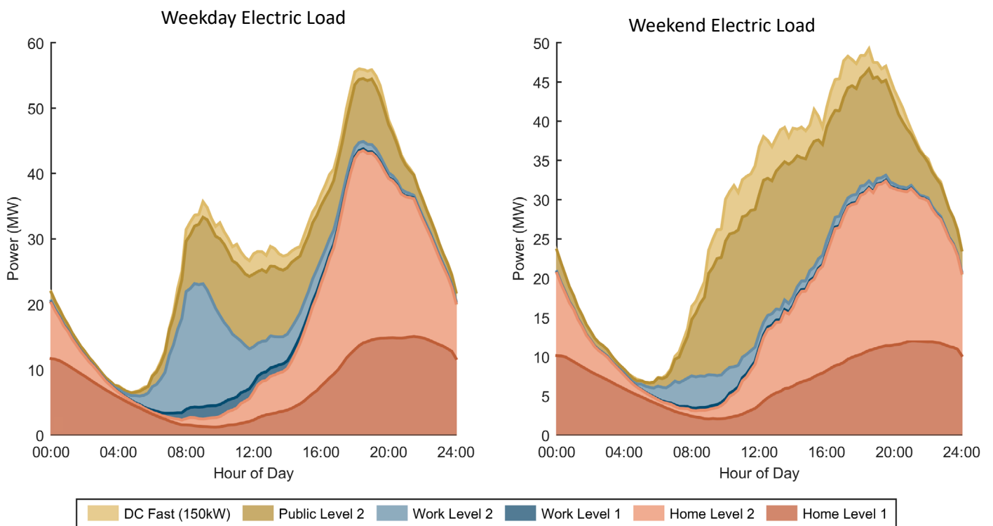
Load Profile for Aggressive EV adoption scenario of Honolulu urban area
