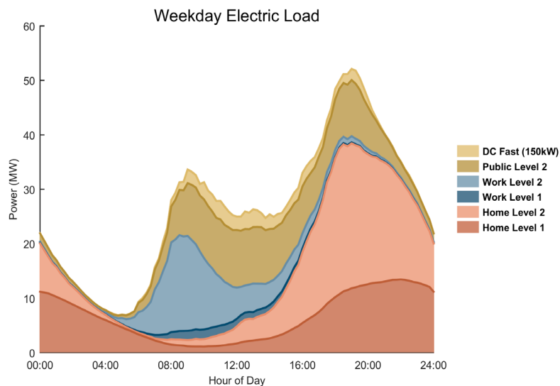
Load Forecasts for Des Moines under an Aggressive Adoption Scenario
