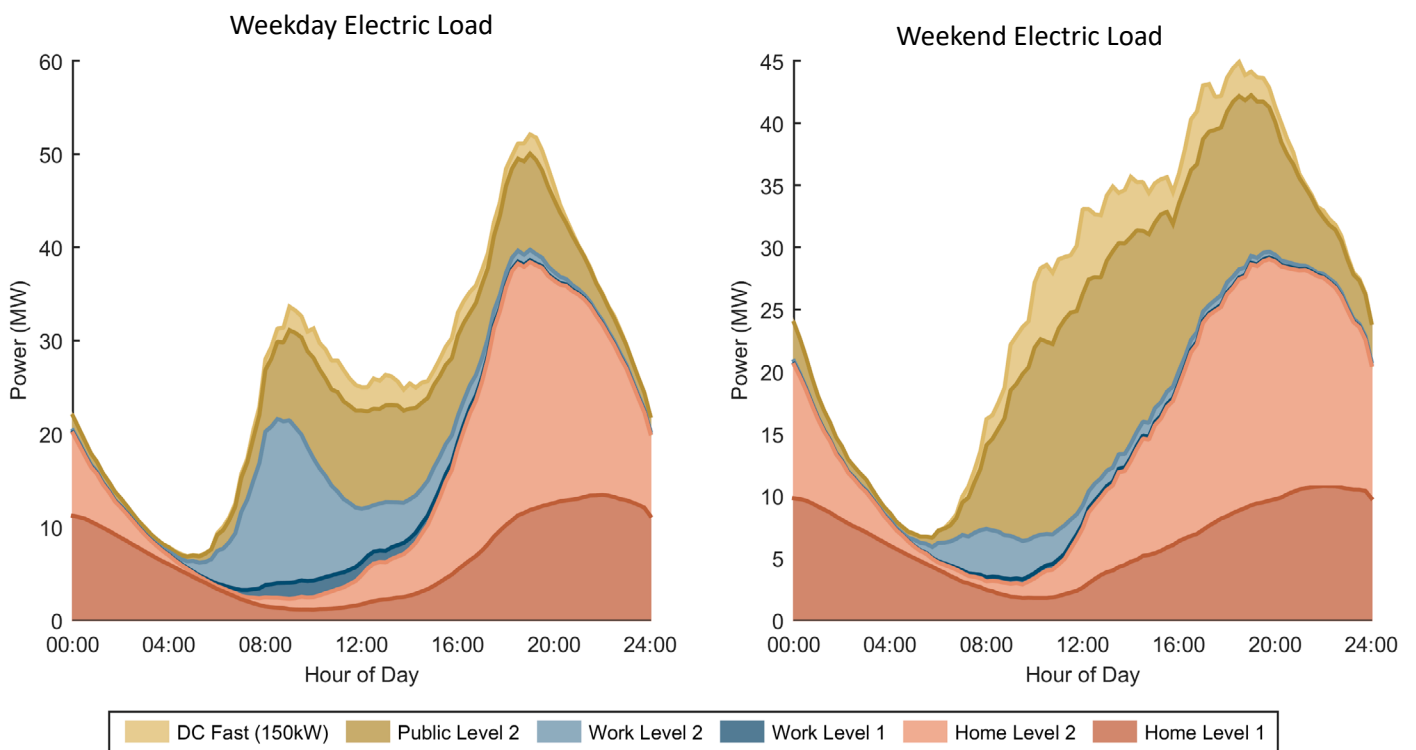
Load Profile for Aggressive EV adoption scenario of Des Moines urban area
