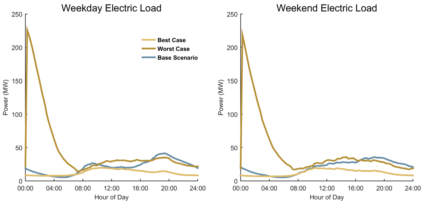
Baseline-, Worst- case, and Best-case load profiles for Aggressive EV adoption for Boise urban area
