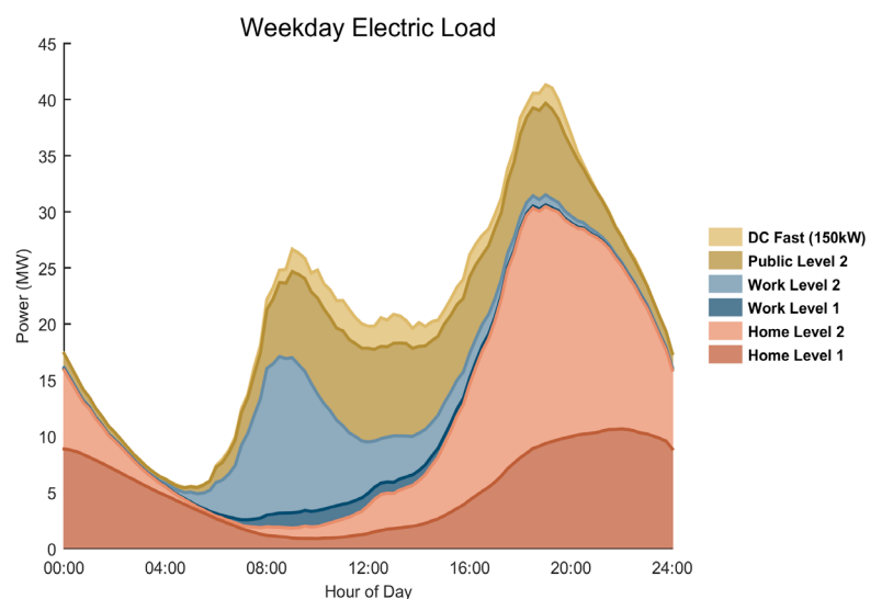
Load Forecasts for Boise under an Aggressive Adoption Scenario
