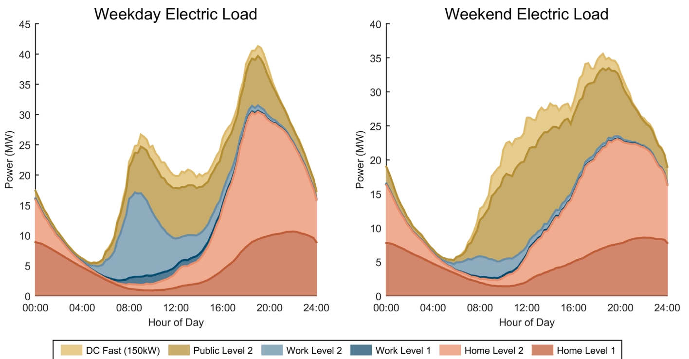
Load Profile for Aggressive EV adoption scenario of Boise urban area
