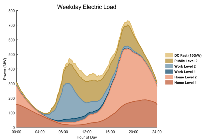
Load Forecasts for Chicago under an Aggressive Adoption Scenario
