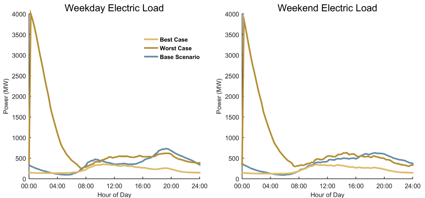
Baseline-, Worst- case, and Best-case load profiles for Aggressive EV adoption for Chicago urban area
