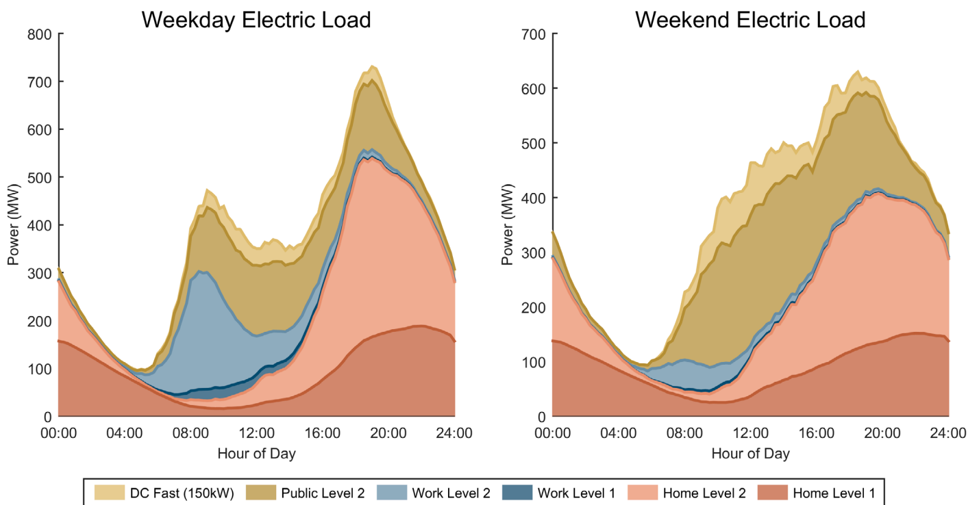
Load Profile for Aggressive EV adoption scenario of Chicago urban area
