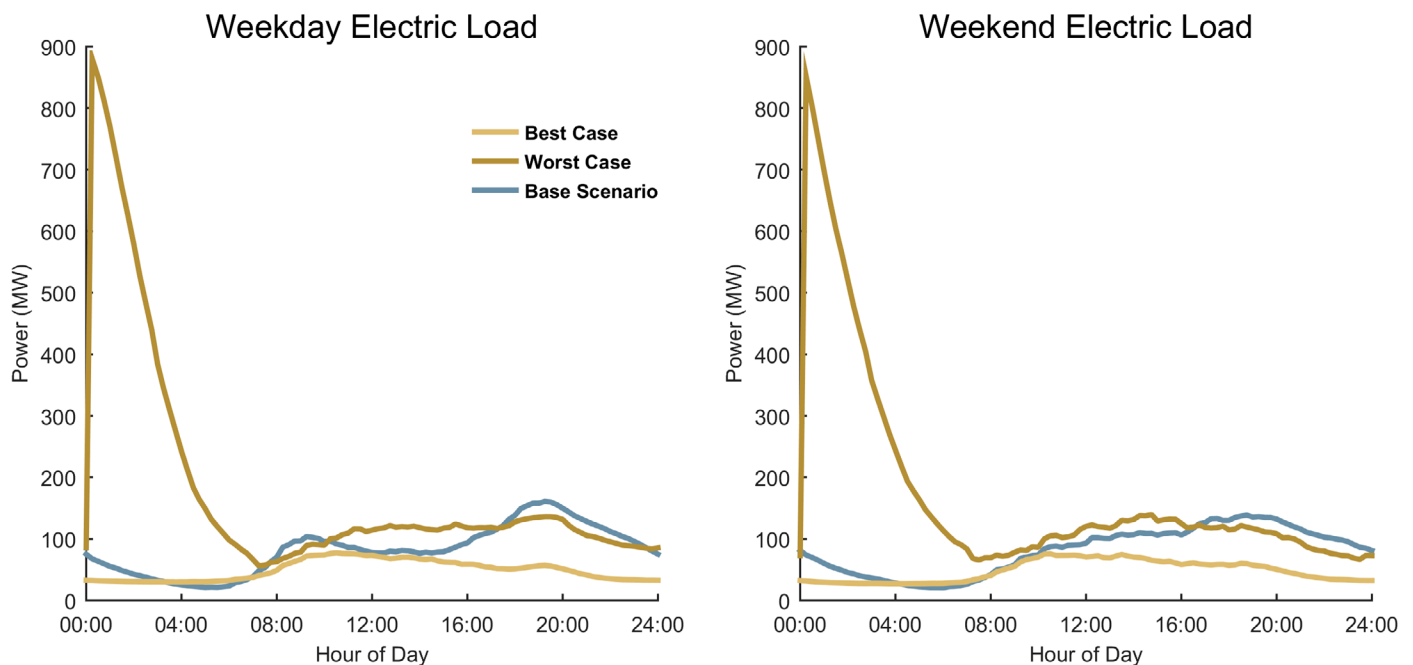
Baseline-, Worst- case, and Best-case load profiles for Aggressive EV adoption for Indianapolis urban area
