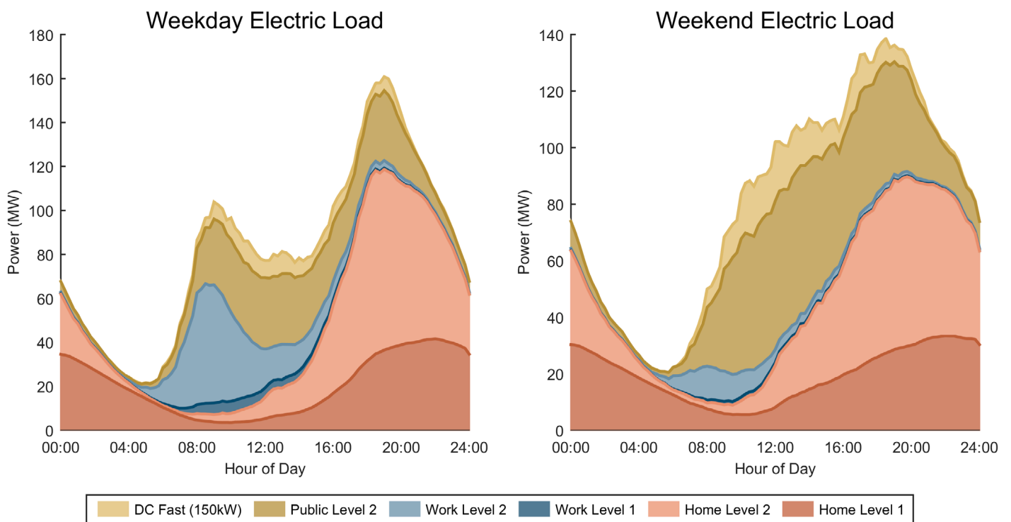
Load Profile for Aggressive EV adoption scenario of Indianapolis urban area
