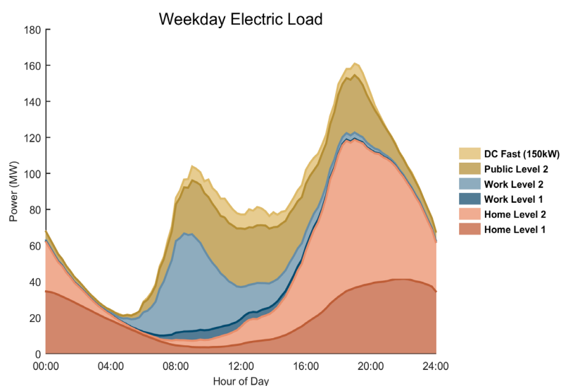
Load Forecasts for Indianapolis under an Aggressive Adoption Scenario
