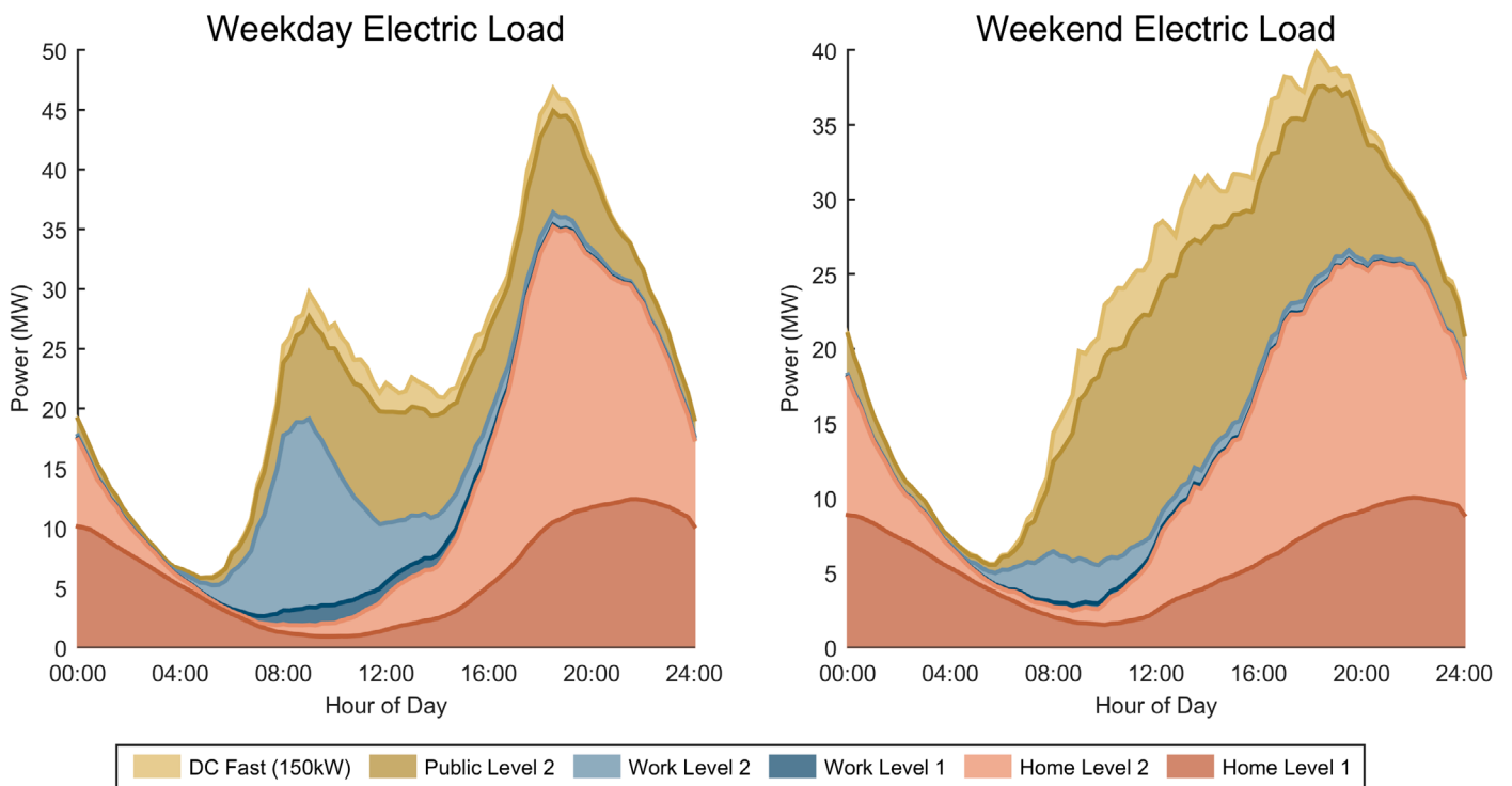
Load Profile for Aggressive EV adoption scenario of Wichita urban area
