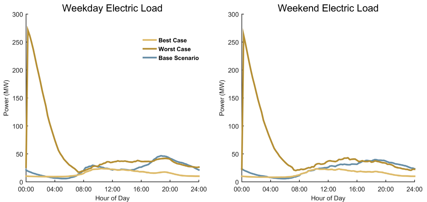
Baseline-, Worst- case, and Best-case load profiles for Aggressive EV adoption for Wichita urban area
