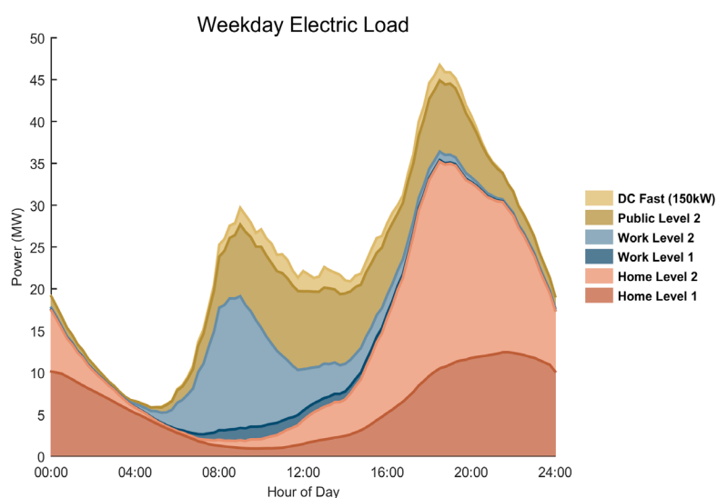
Load Forecasts for Wichita under an Aggressive Adoption Scenario
