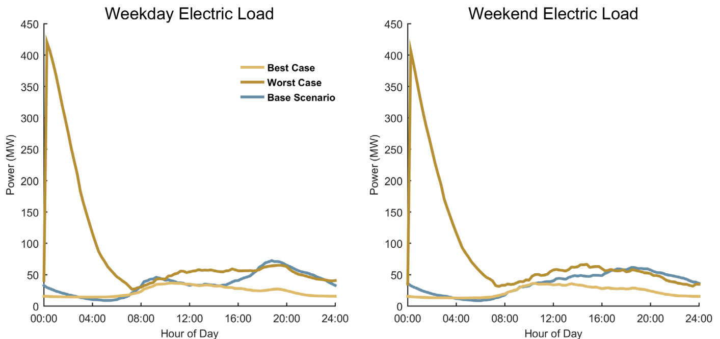
Baseline-, Worst- case, and Best-case load profiles for Aggressive EV adoption for New Orleans urban area
