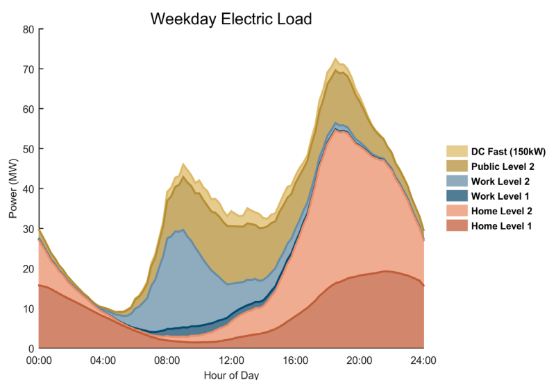
Load Forecasts for New Orleans under an Aggressive Adoption Scenario
