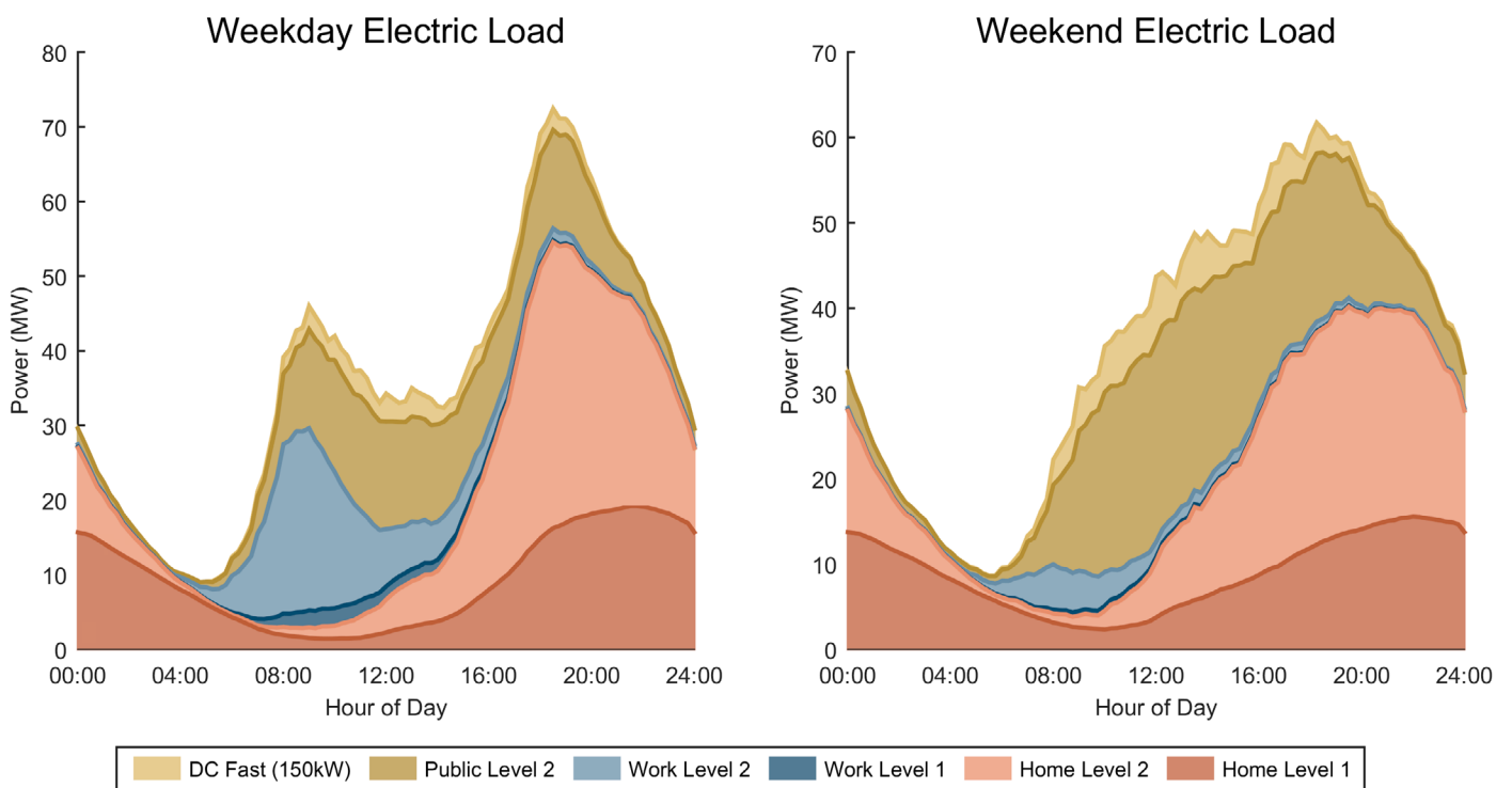
Load Profile for Aggressive EV adoption scenario of New Orleans - Jefferson County urban area
