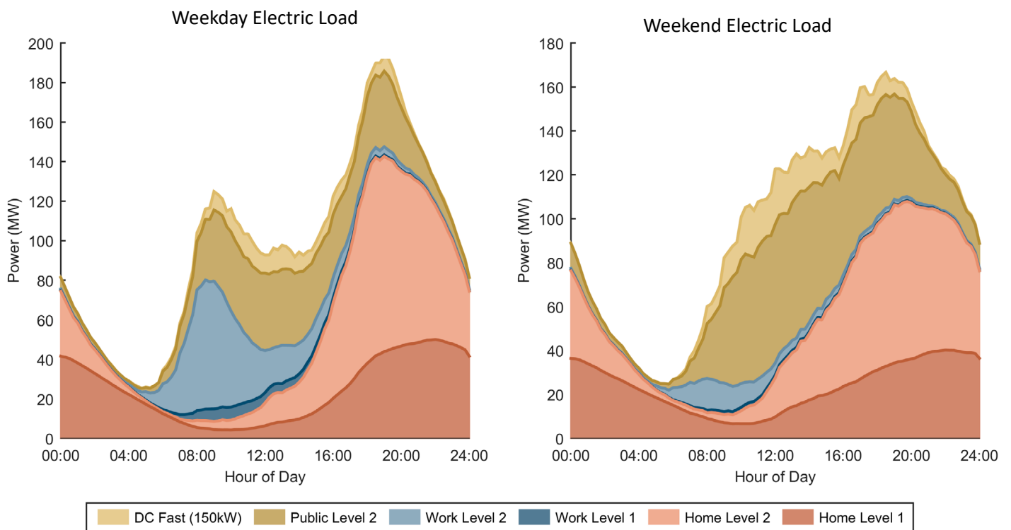
Load Profile for Aggressive EV adoption scenario of Baltimore urban area
