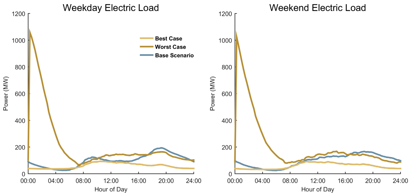
Baseline-, Worst- case, and Best-case load profiles for Aggressive EV adoption for Baltimore urban area
