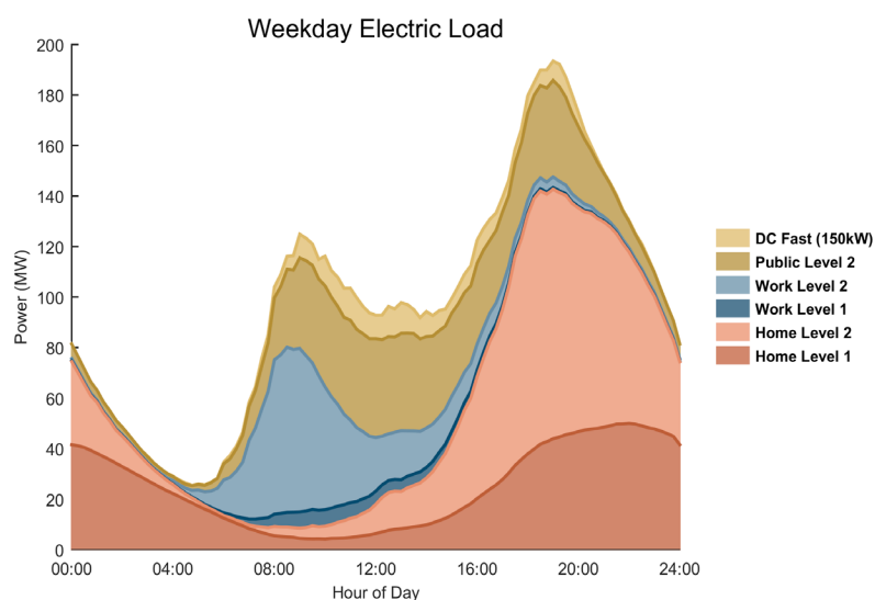
Load Forecasts for Baltimore under an Aggressive Adoption Scenario
