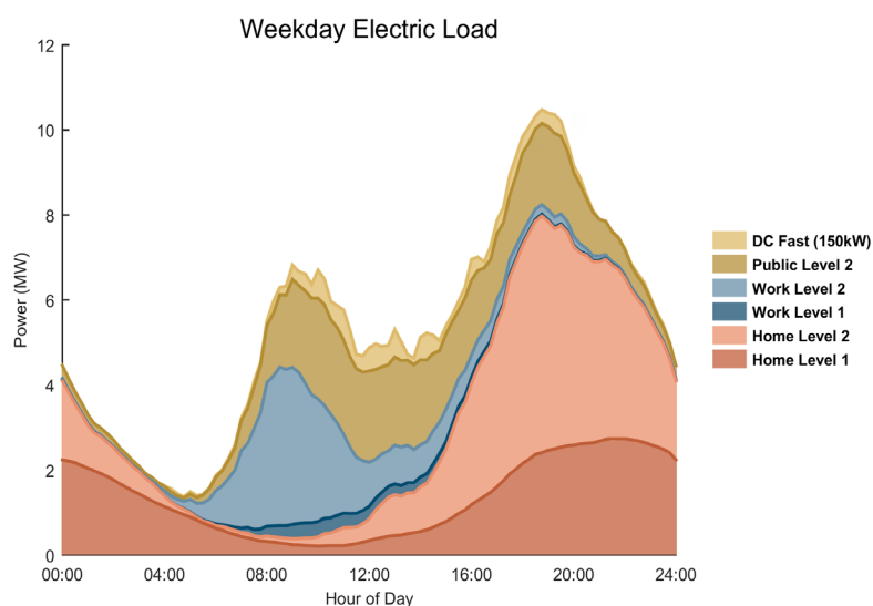
Load Forecasts for Portland under an Aggressive Adoption Scenario
