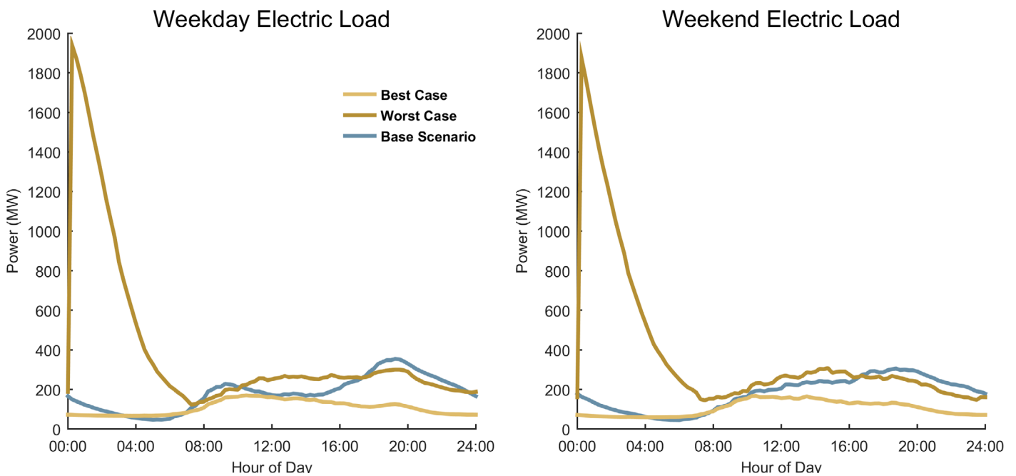
Baseline-, Worst- case, and Best-case load profiles for Aggressive EV adoption for Detroit urban area
