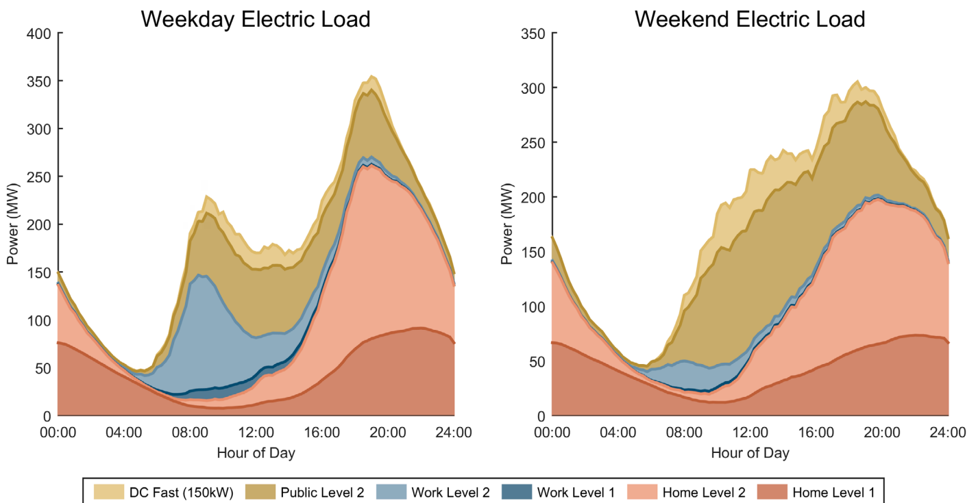
Load Profile for Aggressive EV adoption scenario of Detroit urban area
