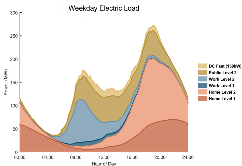
Load Forecasts for Minneapolis under an Aggressive Adoption Scenario
