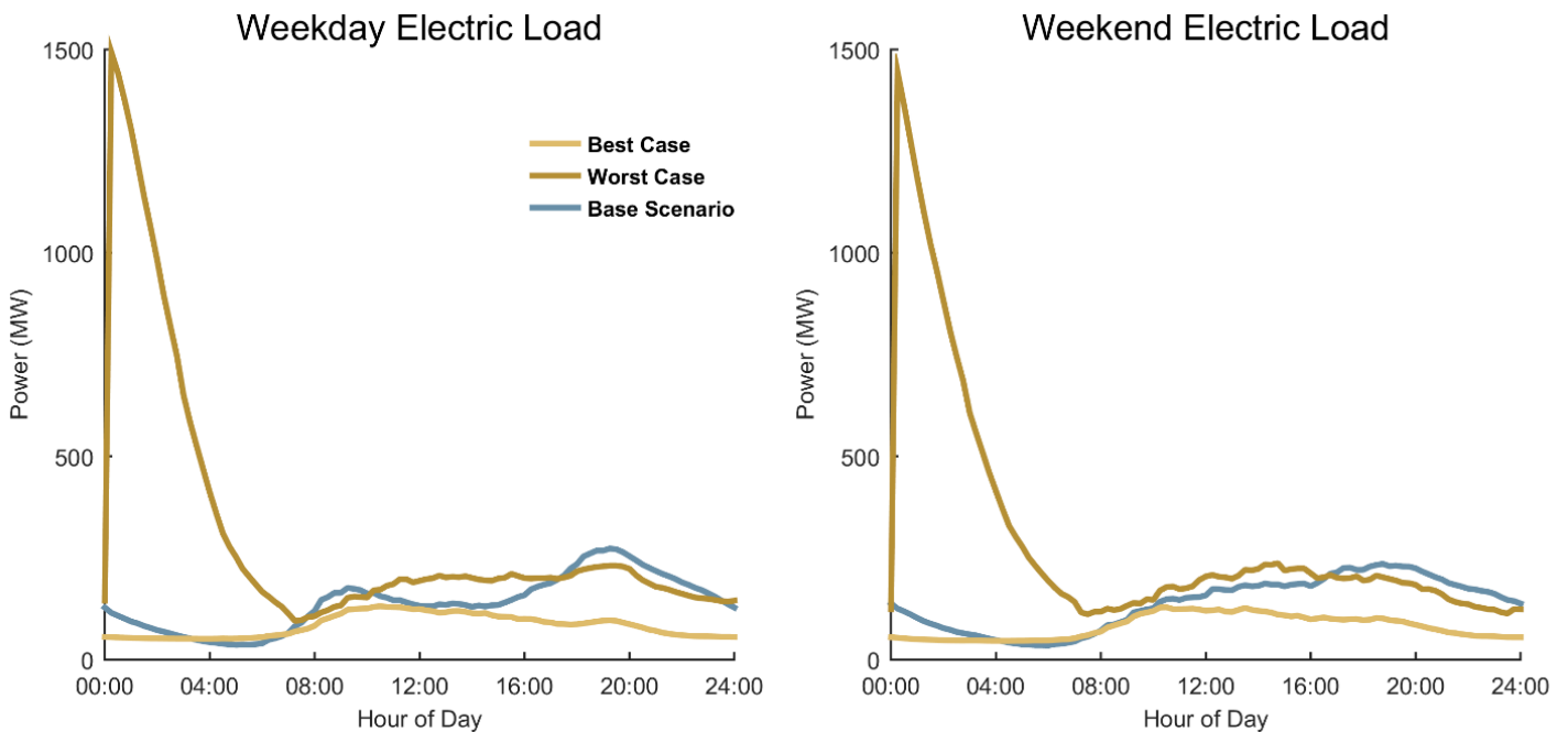
Baseline-, Worst-case, and Best-case load profiles for Aggressive EV adoption for Minneapolis - St. Paul urban area
