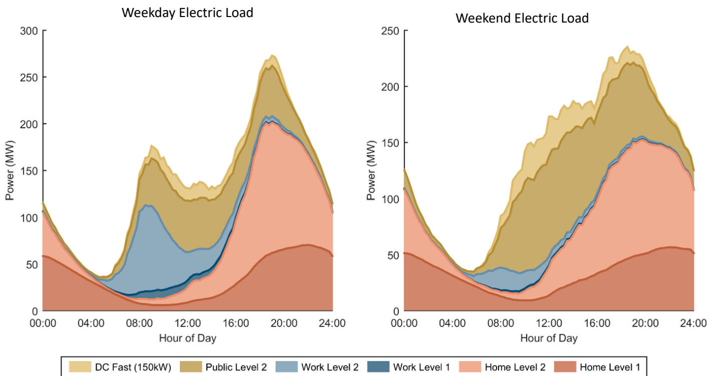
Load Profile for Aggressive EV adoption scenario of Minneapolis - St. Paul urban area
