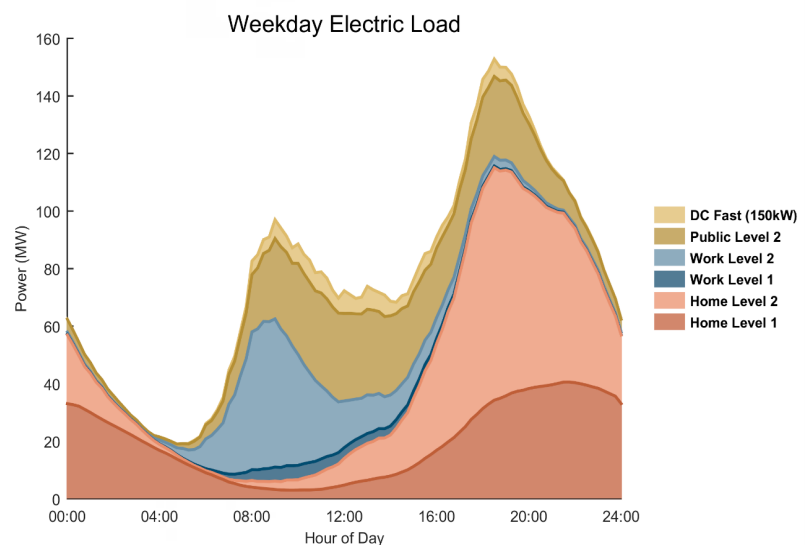
Load Forecasts for Kansas City under an Aggressive Adoption Scenario
