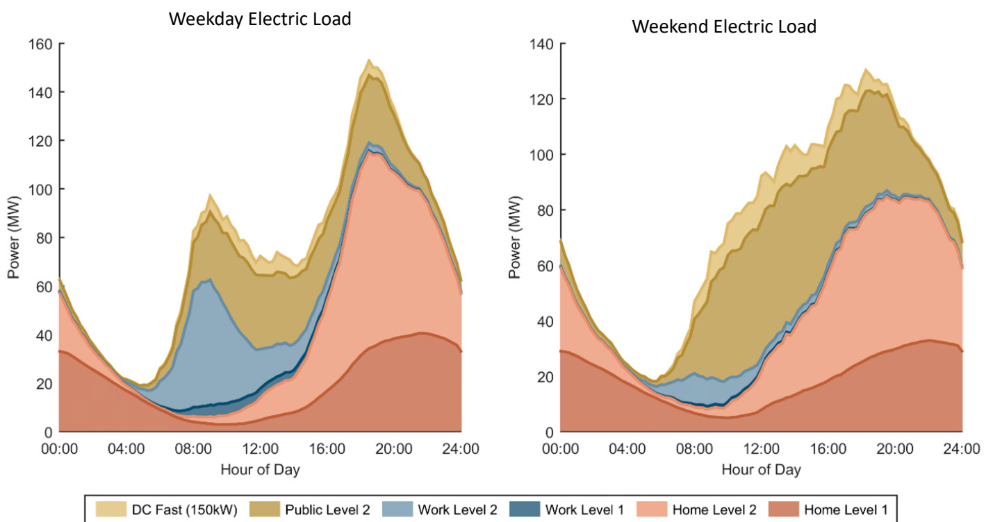
Load Profile for Aggressive EV adoption scenario of Kansas City urban area
