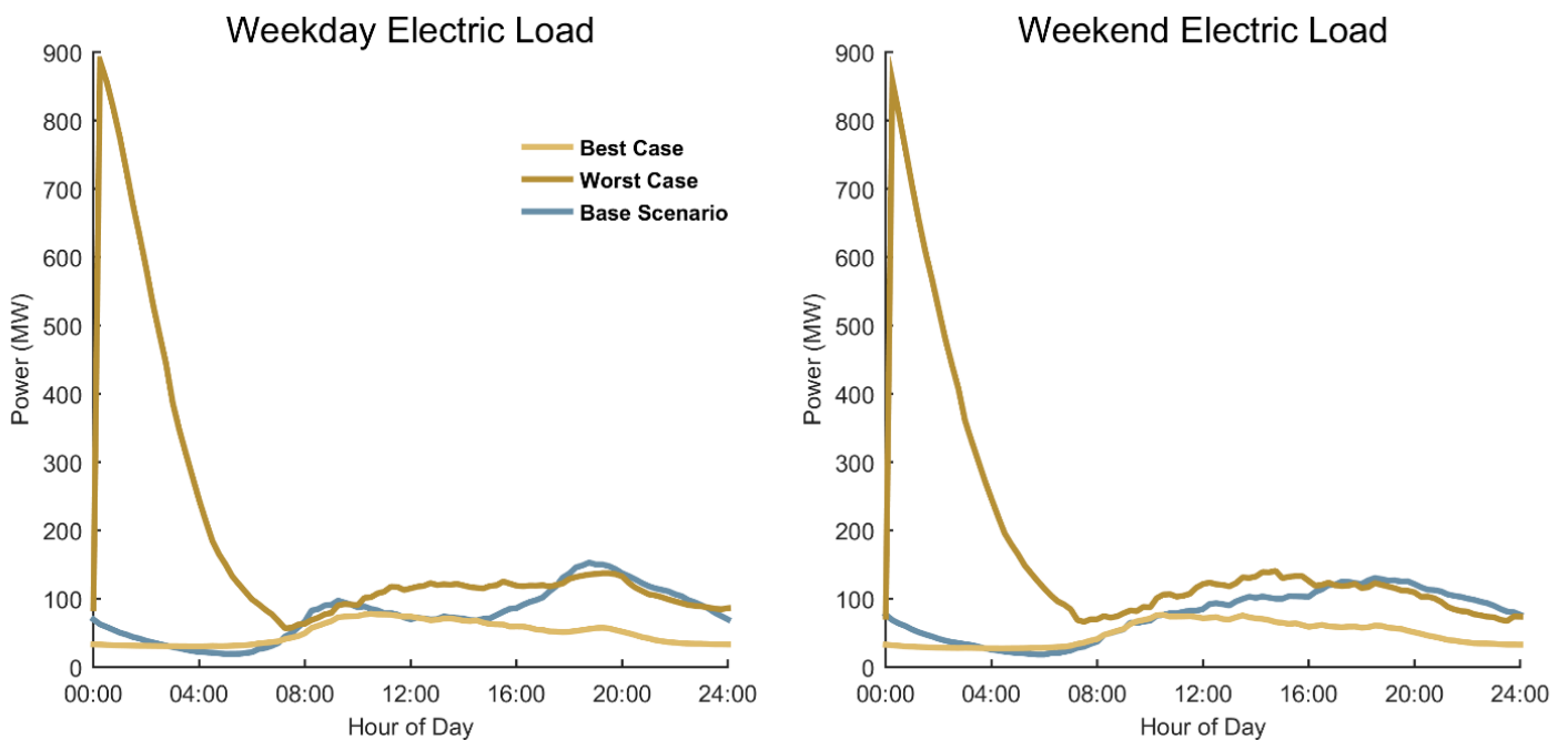
Baseline-, Worst- case, and Best-case load profiles for Aggressive EV adoption for Kansas City urban area
