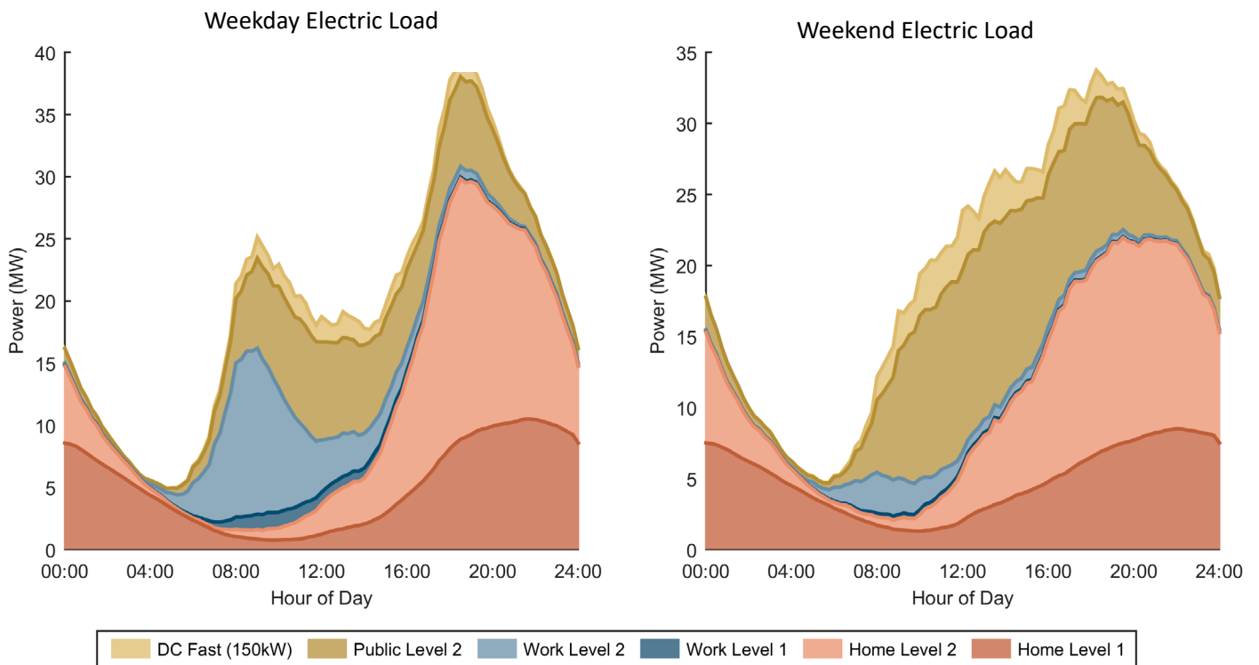
Load Profile for Aggressive EV adoption scenario of Jackson urban area
