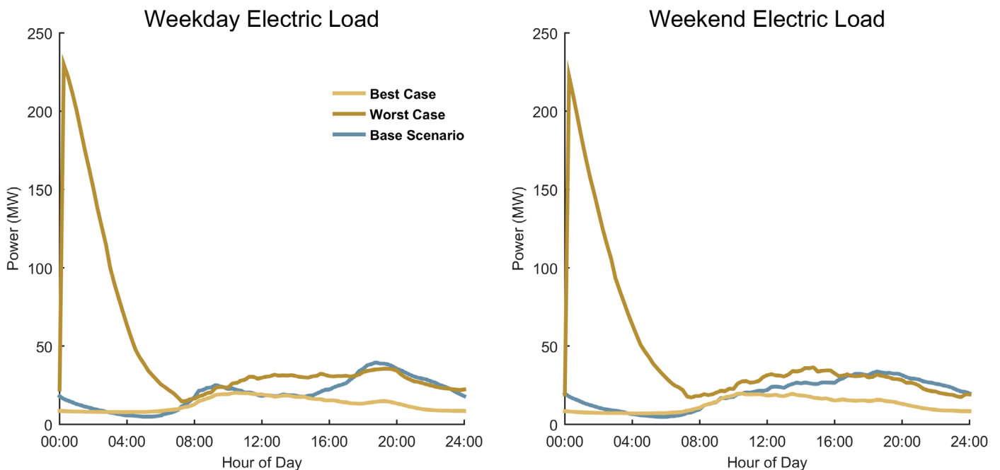
Baseline-, Worst- case, and Best-case load profiles for Aggressive EV adoption for Jackson urban area
