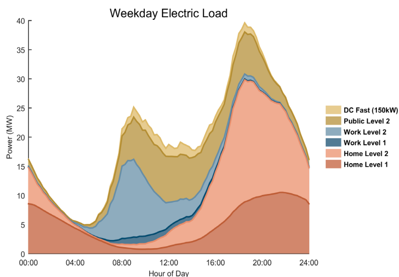
Load Forecasts for Jackson under an Aggressive Adoption Scenario
