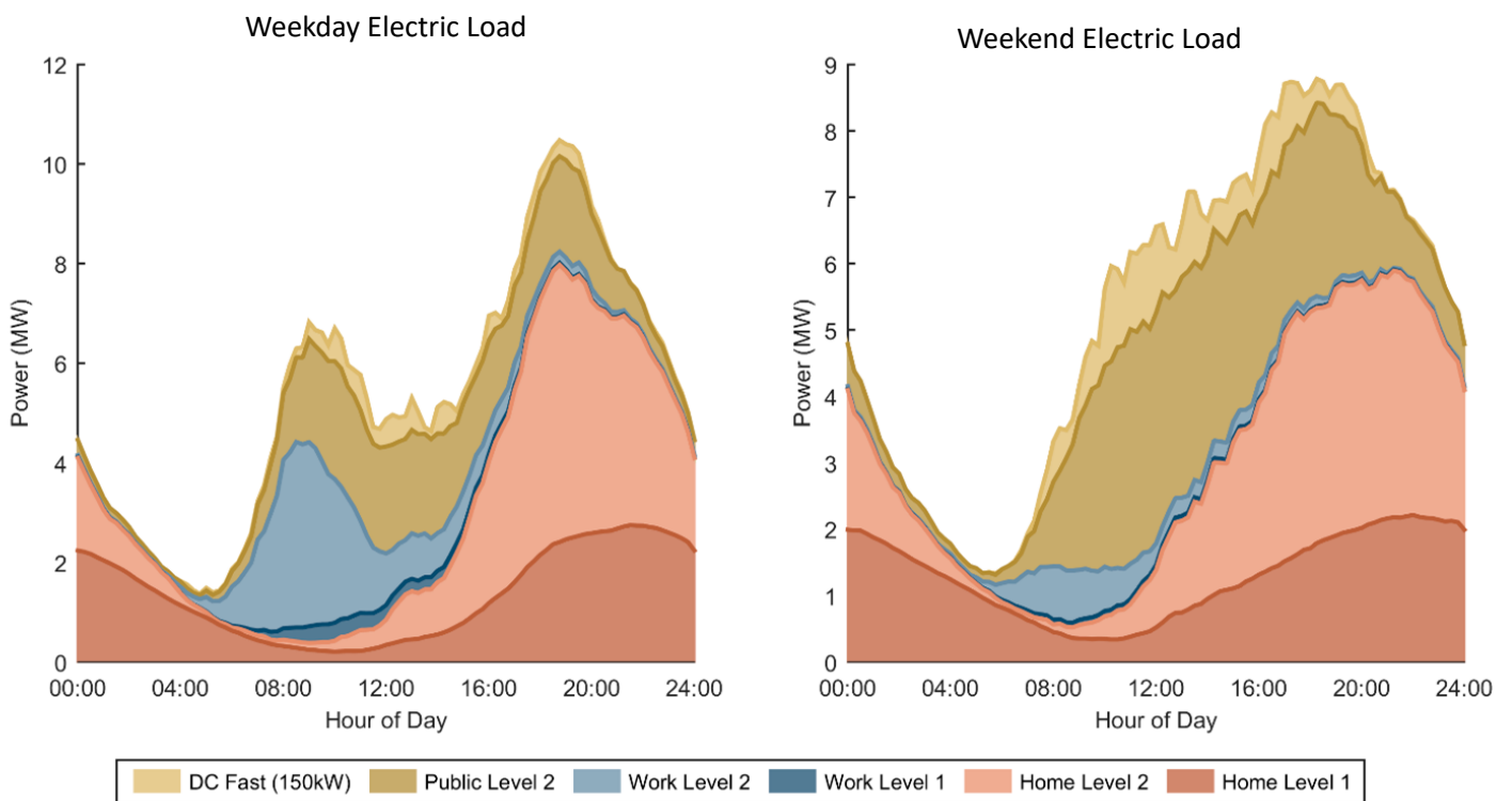
Load Profile for Aggressive EV adoption scenario of Billings urban area
