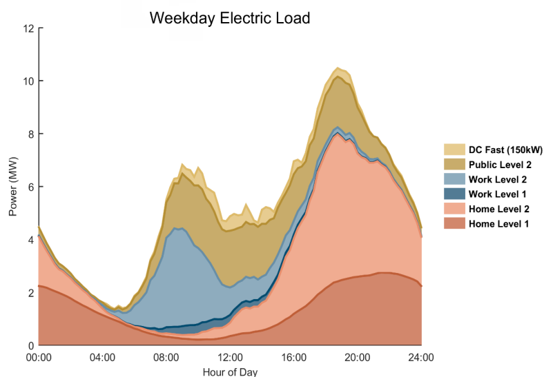
Load Forecasts for Billings under an Aggressive Adoption Scenario
