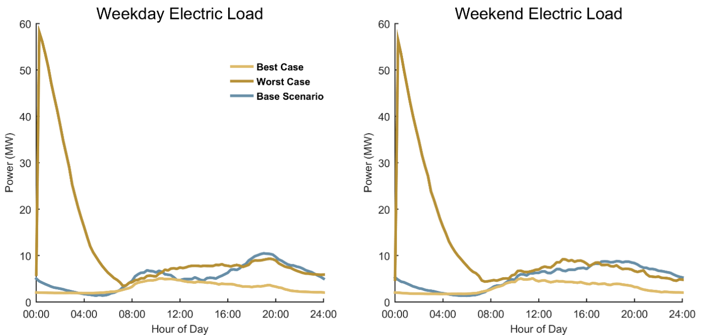
Baseline-, Worst- case, and Best-case load profiles for Aggressive EV adoption for Billings urban area
