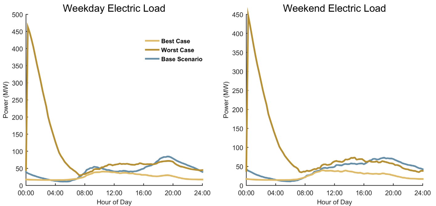
Baseline-, Worst- case, and Best-case load profiles for Aggressive EV adoption for Omaha urban area
