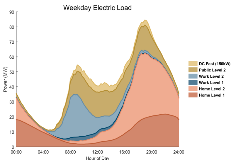
Load Forecasts for Omaha under an Aggressive Adoption Scenario
