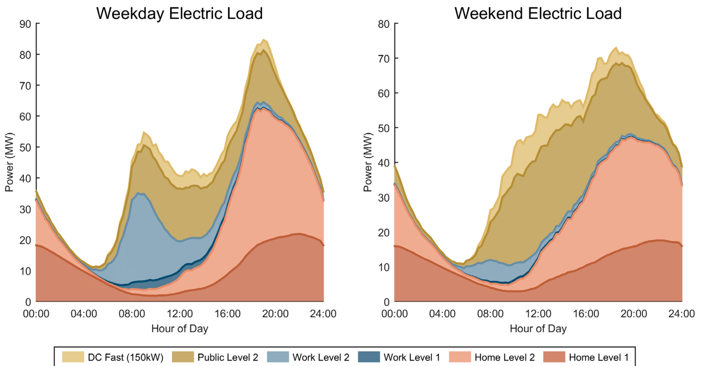
Load Profile for Aggressive EV adoption scenario of Omaha urban area
