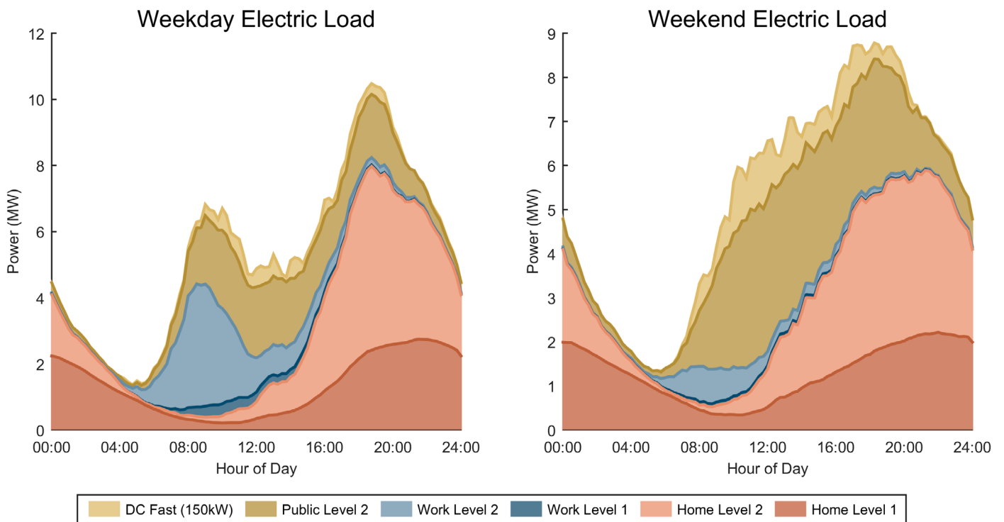
Load Profile for Aggressive EV adoption scenario of Manchester urban area
