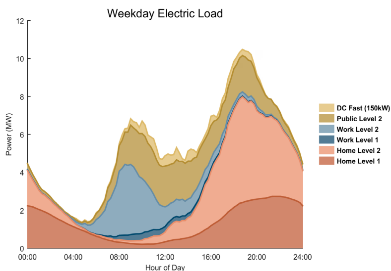
Load Forecasts for Manchester under an Aggressive Adoption Scenario
