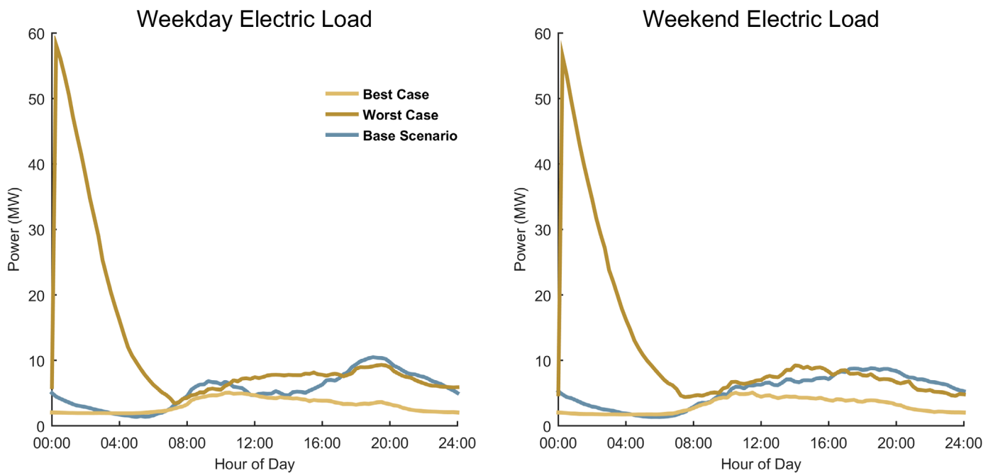
Baseline-, Worst- case, and Best-case load profiles for Aggressive EV adoption for Trenton urban area
