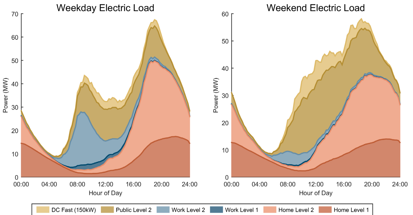
Load Profile for Aggressive EV adoption scenario of Albuquerque urban area
