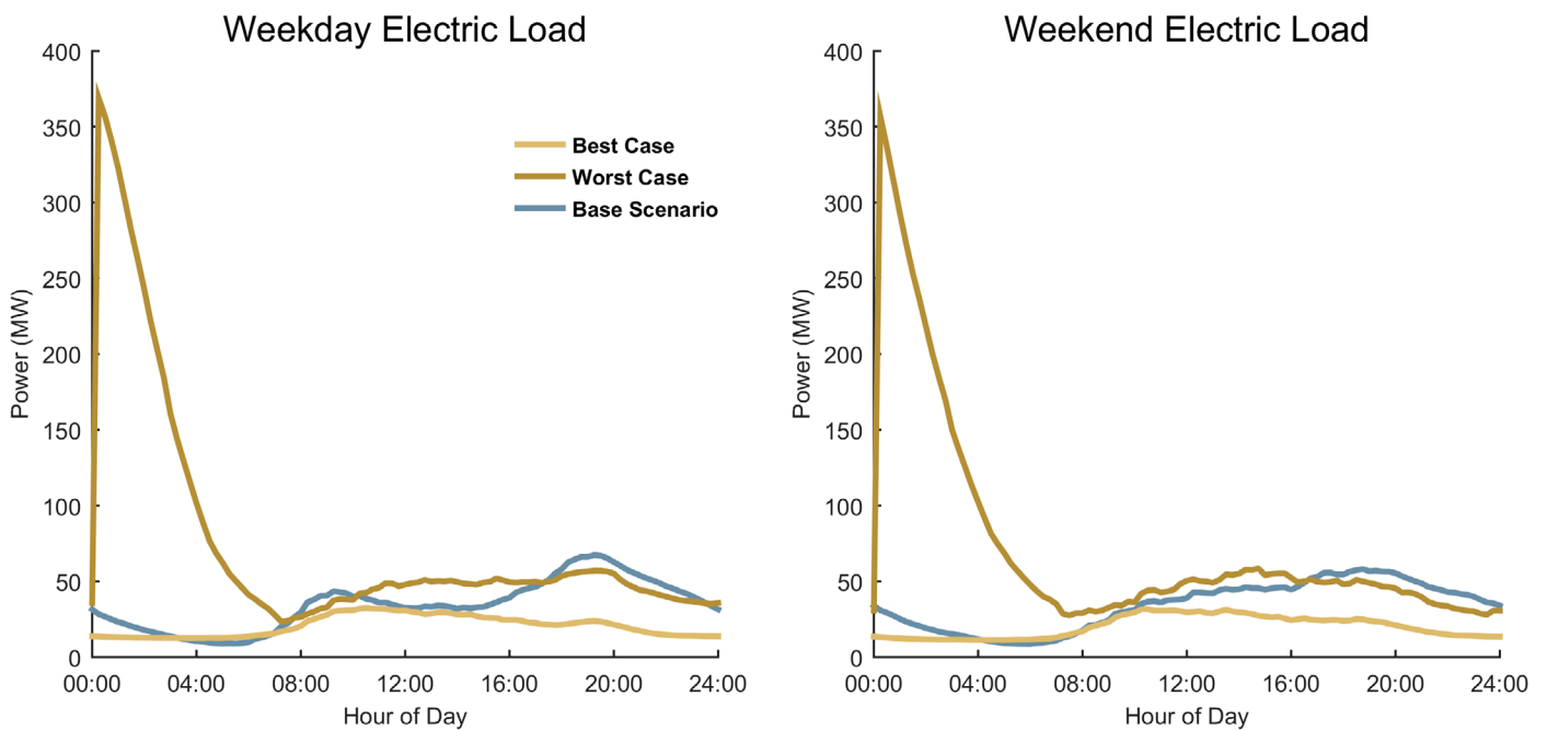
Baseline-, Worst- case, and Best-case load profiles for Aggressive EV adoption for Albuquerque urban area
