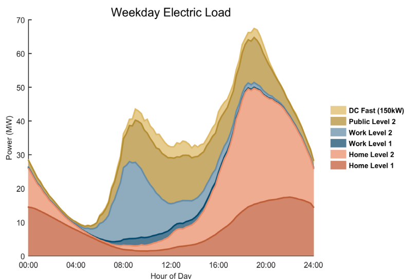
Load Forecasts for Albuquerque under an Aggressive Adoption Scenario
