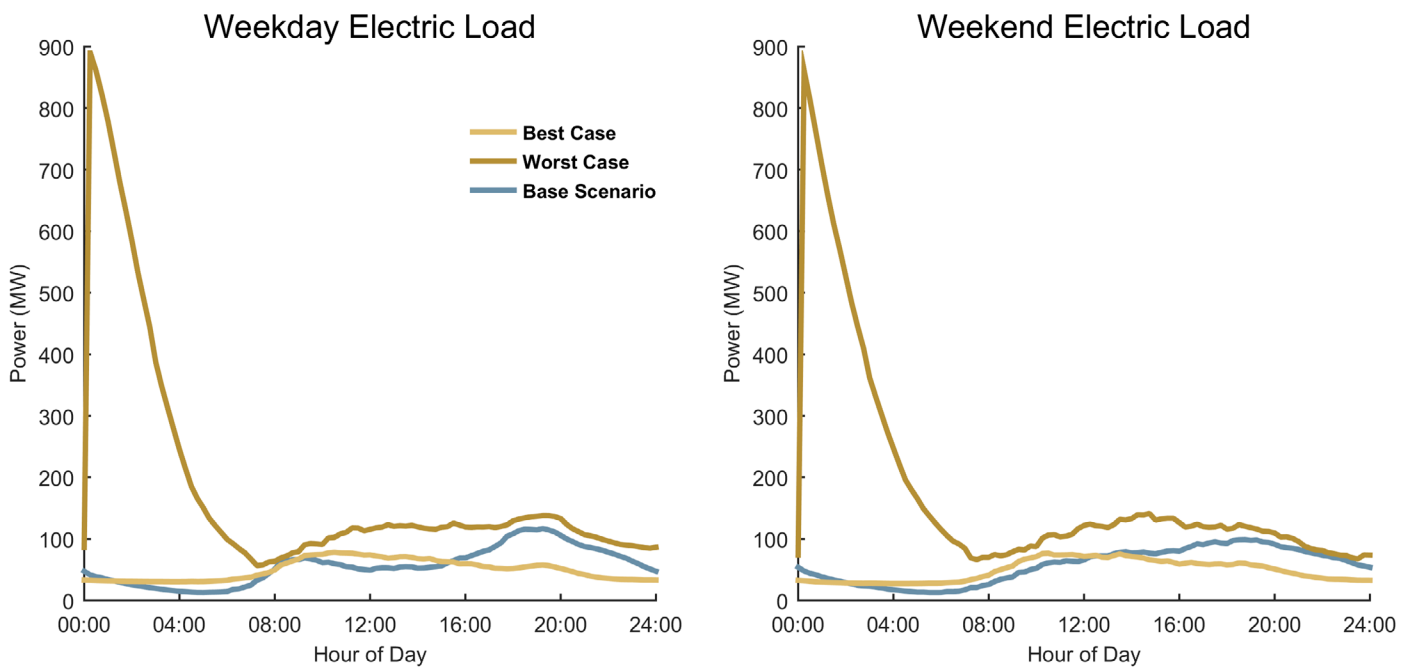
Baseline-, Worst-case, and Best-case load profiles for Aggressive EV adoption for Las Vegas - Henderson urban area
