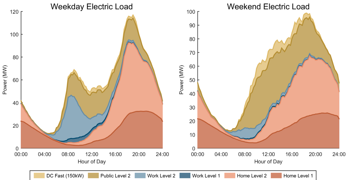
Load Profile for Aggressive EV adoption scenario of Las Vegas - Henderson urban area
