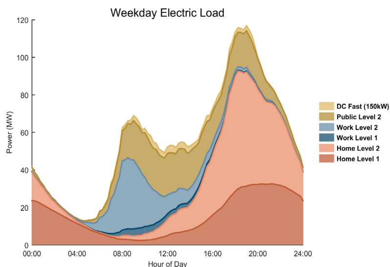
Load Forecasts for Las Vegas under an Aggressive Adoption Scenario
