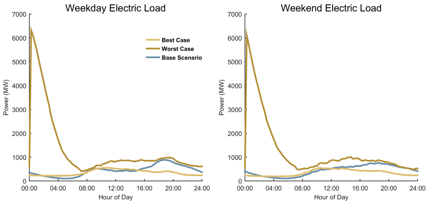
Baseline-, Worst-case, and Best-case load profiles for Aggressive EV adoption for New York urban area
