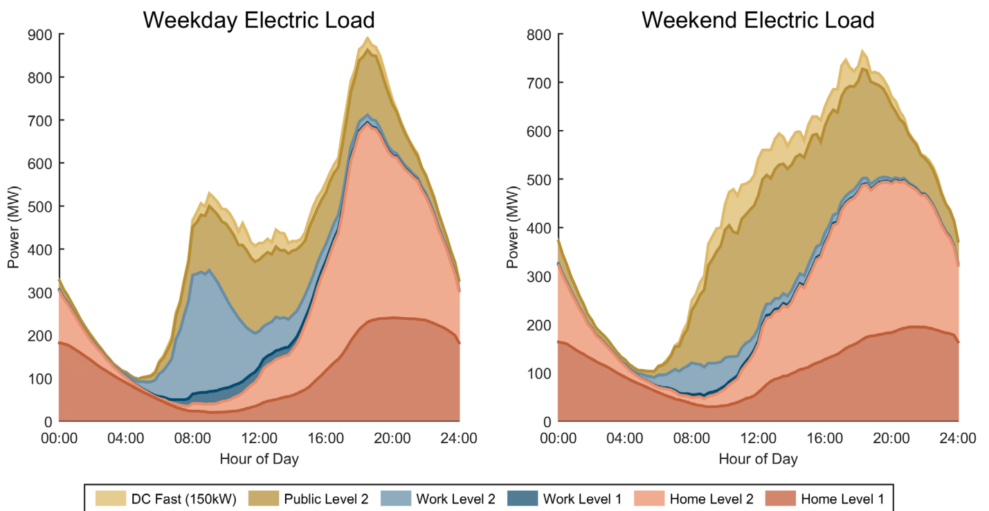
Load Profile for Aggressive EV adoption scenario of New York - Newark urban area
