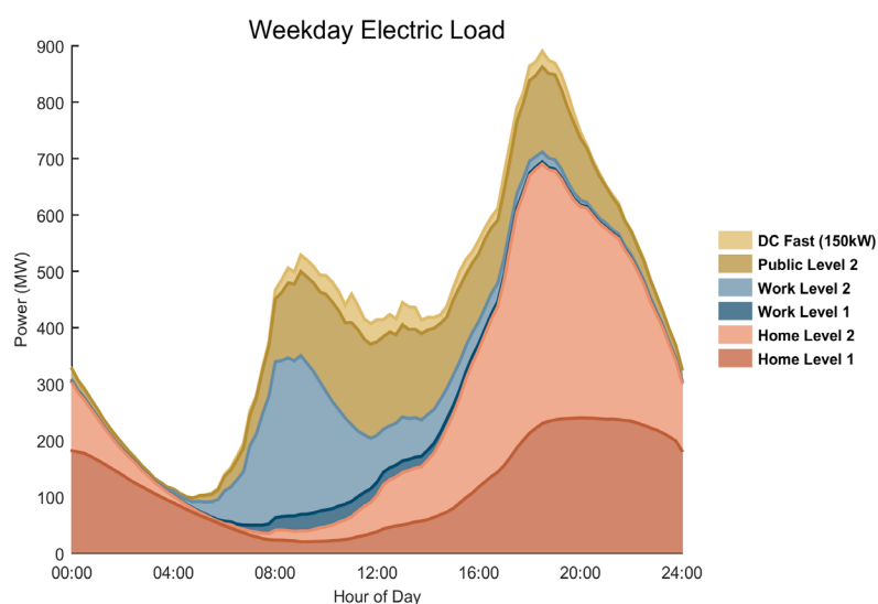
Load Forecasts for New York under an Aggressive Adoption Scenario
