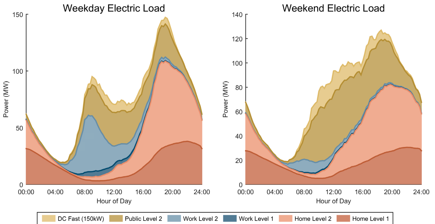
Load Profile for Aggressive EV adoption scenario of Columbus urban area
