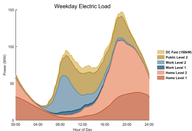
Load Forecasts for Columbus under an Aggressive Adoption Scenario
