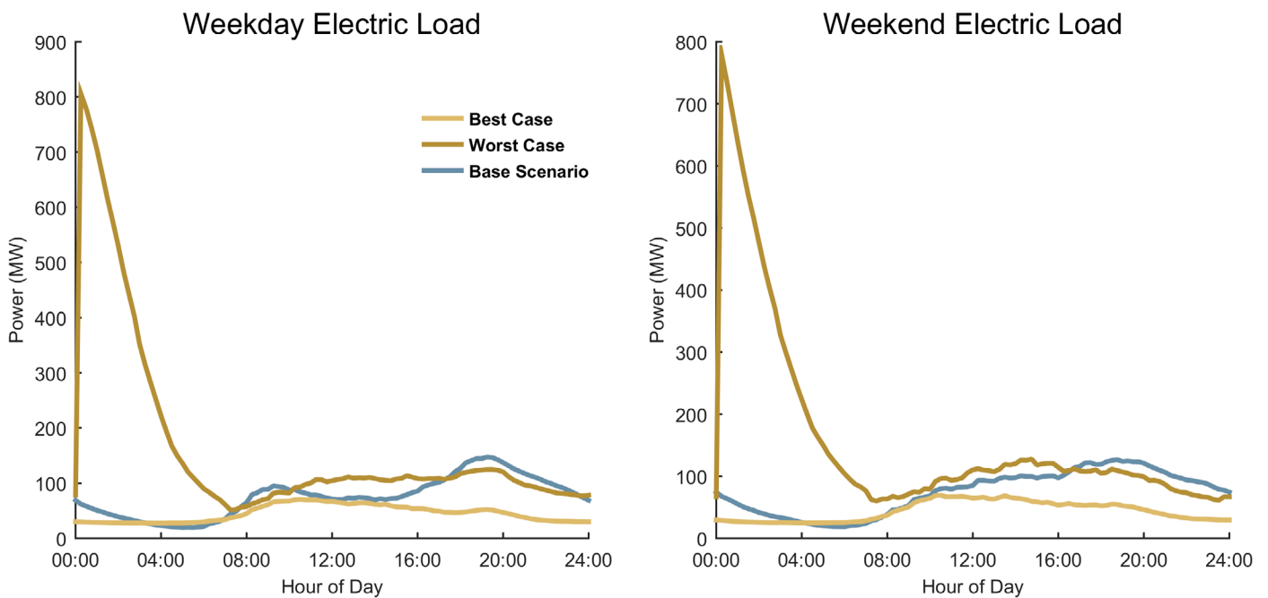
Baseline-, Worst- case, and Best-case load profiles for Aggressive EV adoption for Columbus urban area
