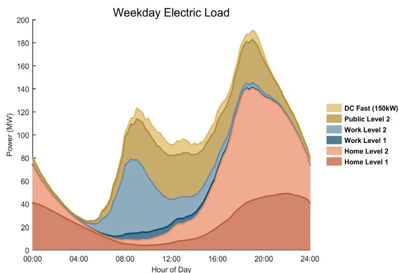
Load Forecasts for Portland under an Aggressive Adoption Scenario
