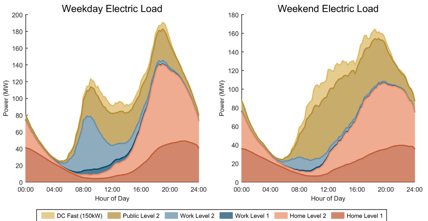
Load Profile for Aggressive EV adoption scenario of Portland urban area
