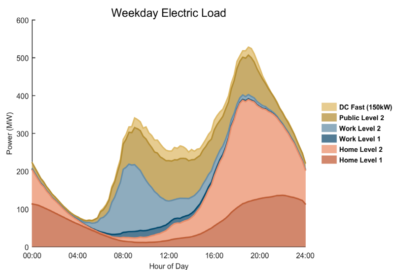
Load Forecasts for Philadelphia under an Aggressive Adoption Scenario
