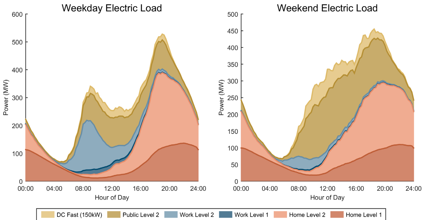
Load Profile for Aggressive EV adoption scenario of Philadelphia urban area
