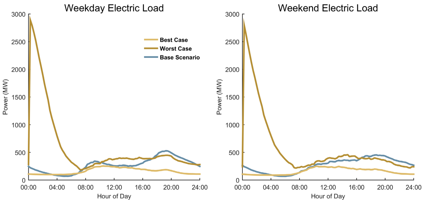
Baseline-, Worst- case, and Best-case load profiles for Aggressive EV adoption for Philadelphia urban area
