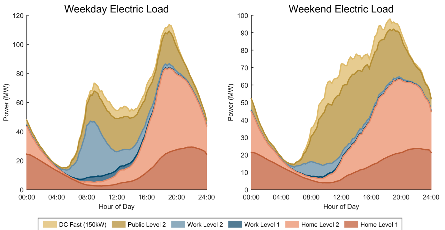
Load Profile for Aggressive EV adoption scenario of Providence urban area
