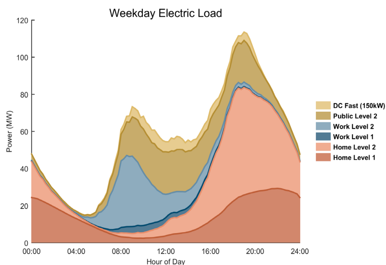
Load Forecasts for Providence under an Aggressive Adoption Scenario
