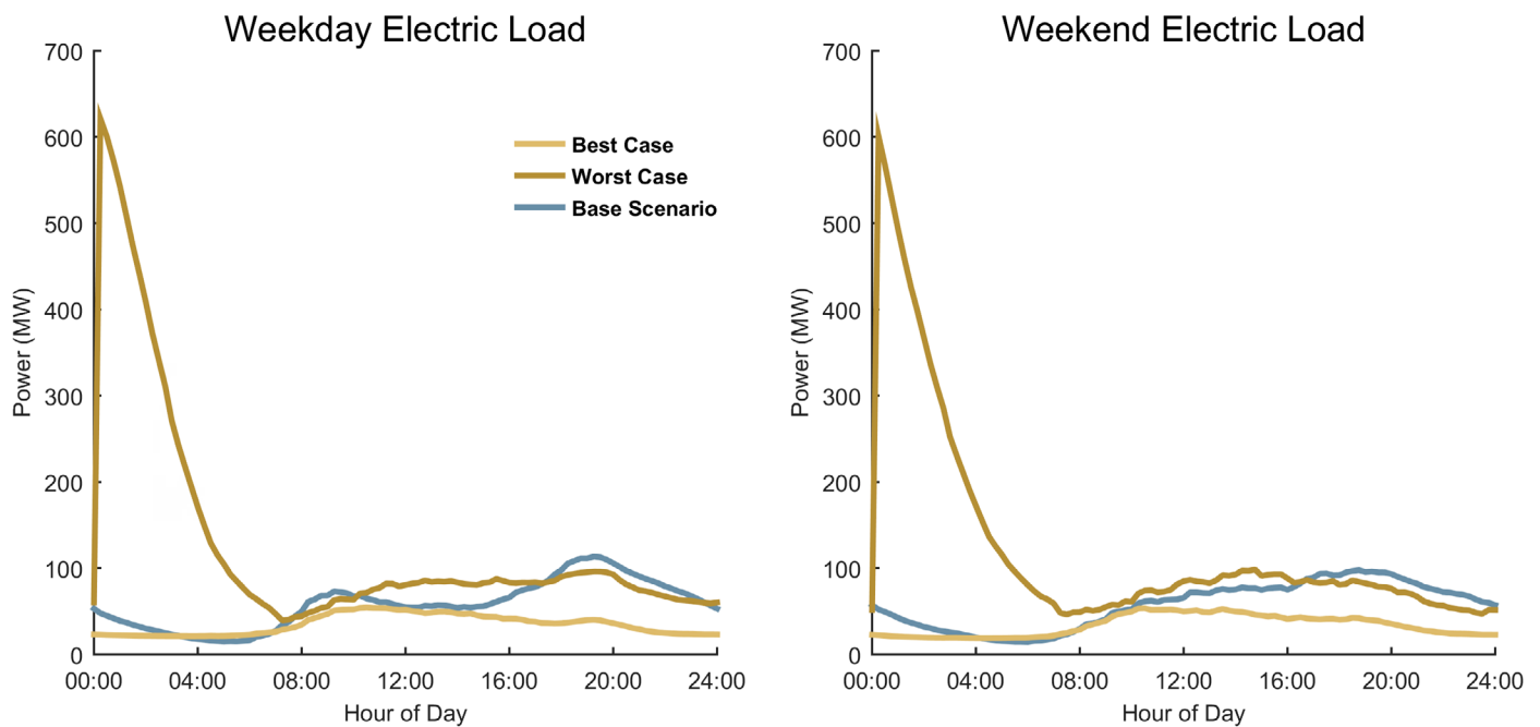
Baseline-, Worst- case, and Best-case load profiles for Aggressive EV adoption for Providence urban area
