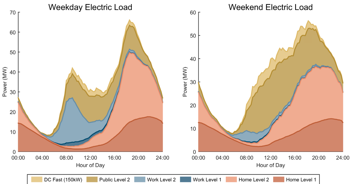
Load Profile for Aggressive EV adoption scenario of Charleston - North Charleston urban area
