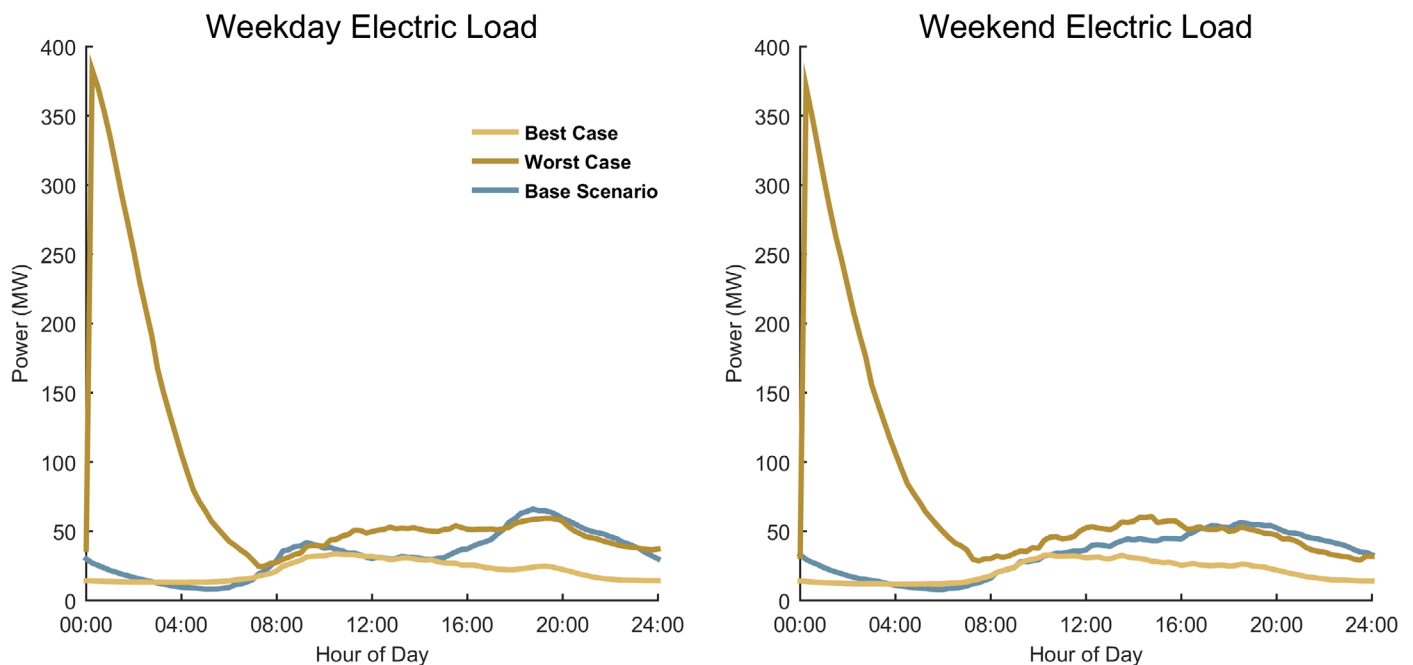
Baseline-, Worst- case, and Best-case load profiles for Aggressive EV adoption for Charleston - North Charleston urban area
