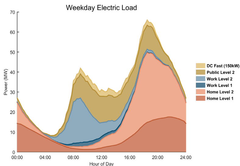
Load Forecasts for Charleston under an Aggressive Adoption Scenario
