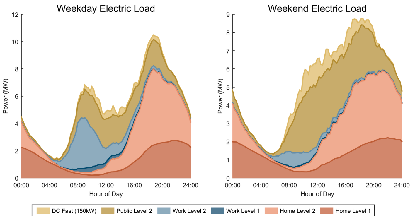
Load Profile for Aggressive EV adoption scenario of Sioux Falls urban area
