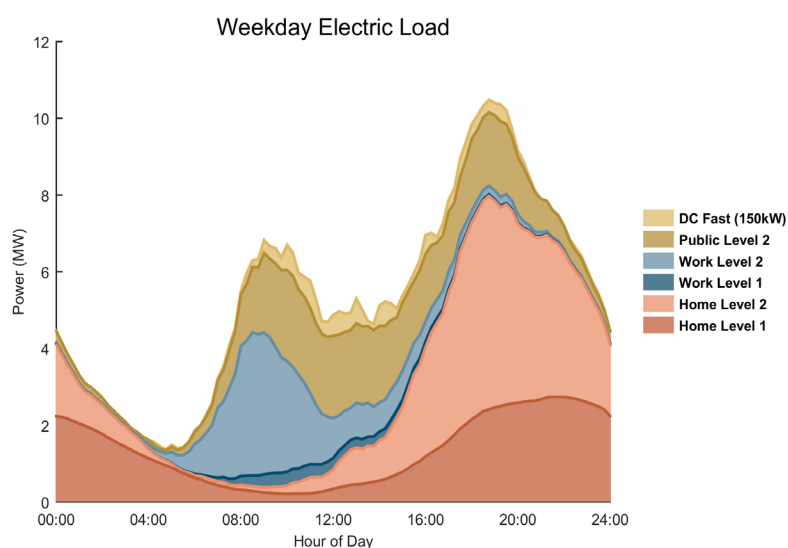
Load Forecasts for Sioux Falls under an Aggressive Adoption Scenario
