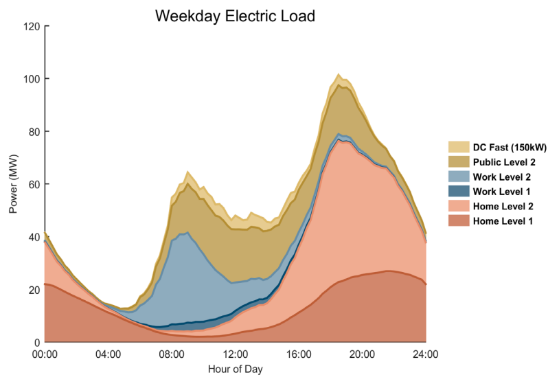
Load Forecasts for Nashville under an Aggressive Adoption Scenario
