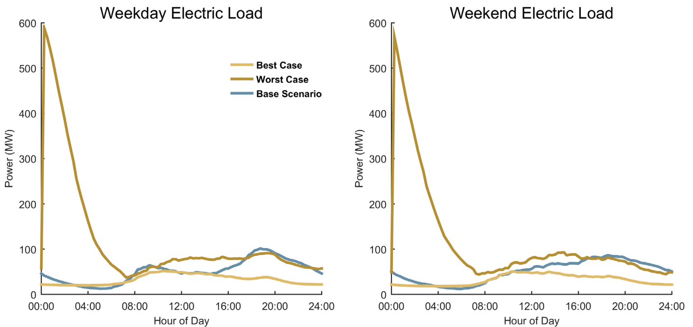
Baseline-, Worst- case, and Best-case load profiles for Aggressive EV adoption for Nashville-Davidson urban area
