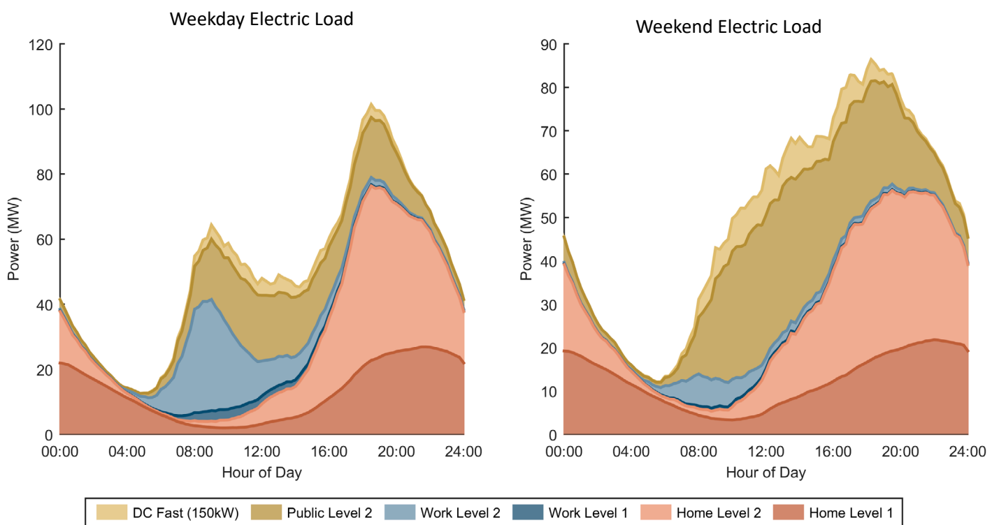
Load Profile for Aggressive EV adoption scenario of Nashville-Davidson urban area
