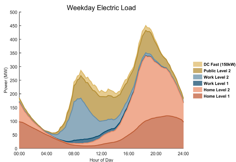
Load Forecasts for Houston under an Aggressive Adoption Scenario
