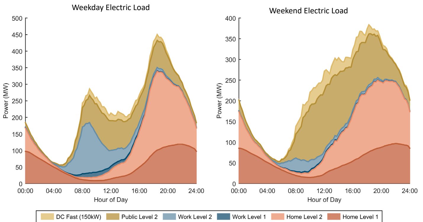
Load Profile for Aggressive EV adoption scenario of Houston urban area
