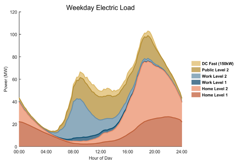
Load Forecasts for Salt Lake City under an Aggressive Adoption Scenario
