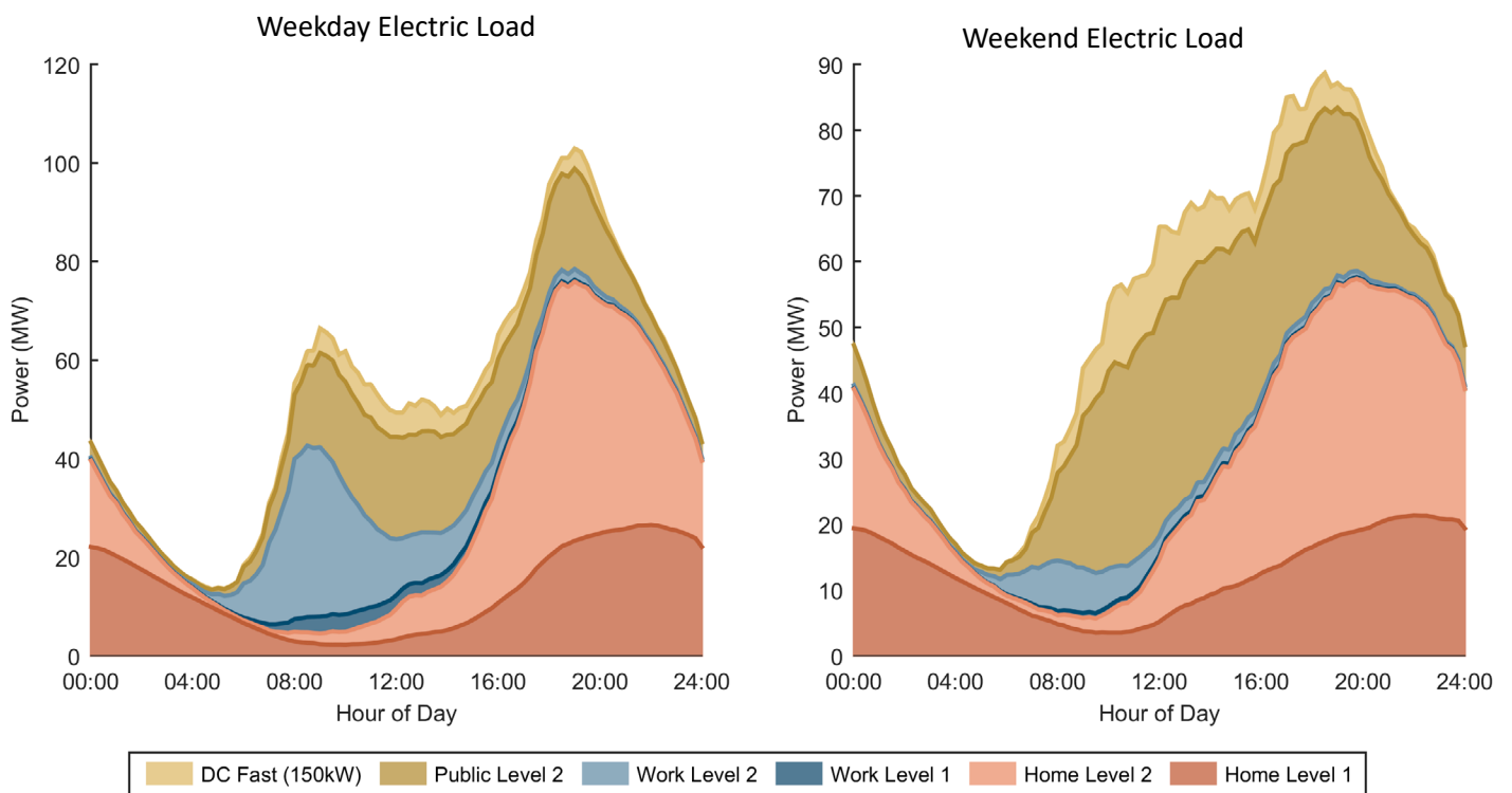
Load Profile for Aggressive EV adoption scenario of Salt Lake City - West Valley City urban area
