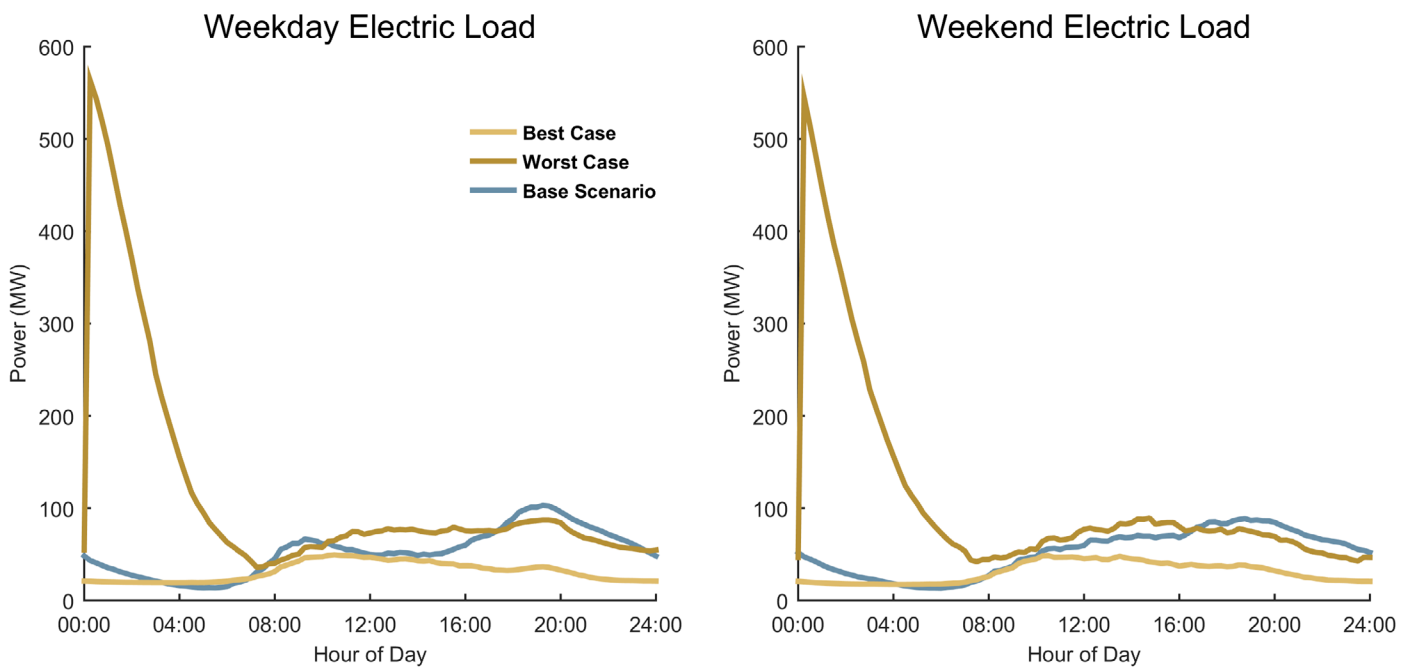
Baseline-, Worst- case, and Best-case load profiles for Aggressive EV adoption for Salt Lake City - West Valley City urban area
