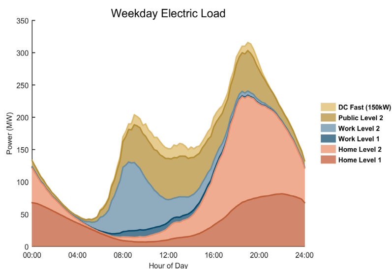
Load Forecasts for Seattle under an Aggressive Adoption Scenario
