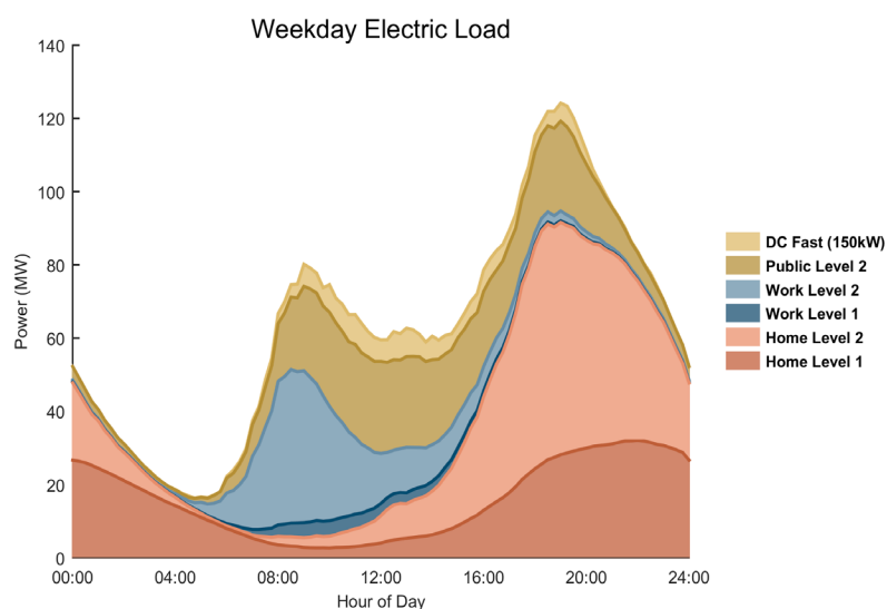
Load Forecasts for Milwaukee under an Aggressive Adoption Scenario
