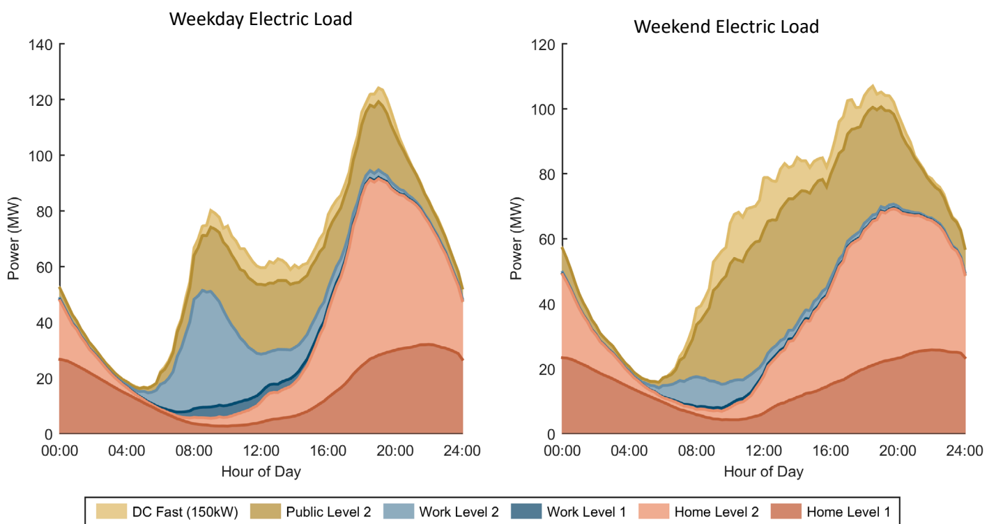
Load Profile for Aggressive EV adoption scenario of Milwaukee urban area
