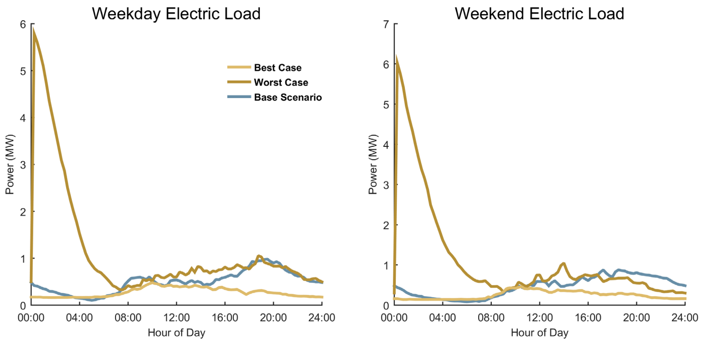
Baseline-, Worst- case, and Best-case load profiles for Aggressive EV adoption for Cheyenne urban area
