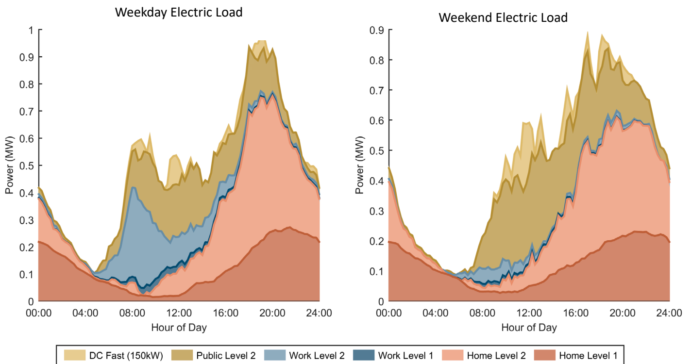
Load Profile for Aggressive EV adoption scenario of Cheyenne urban area
