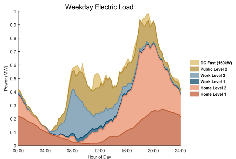
Load Forecasts for Cheyenne under an Aggressive Adoption Scenario
