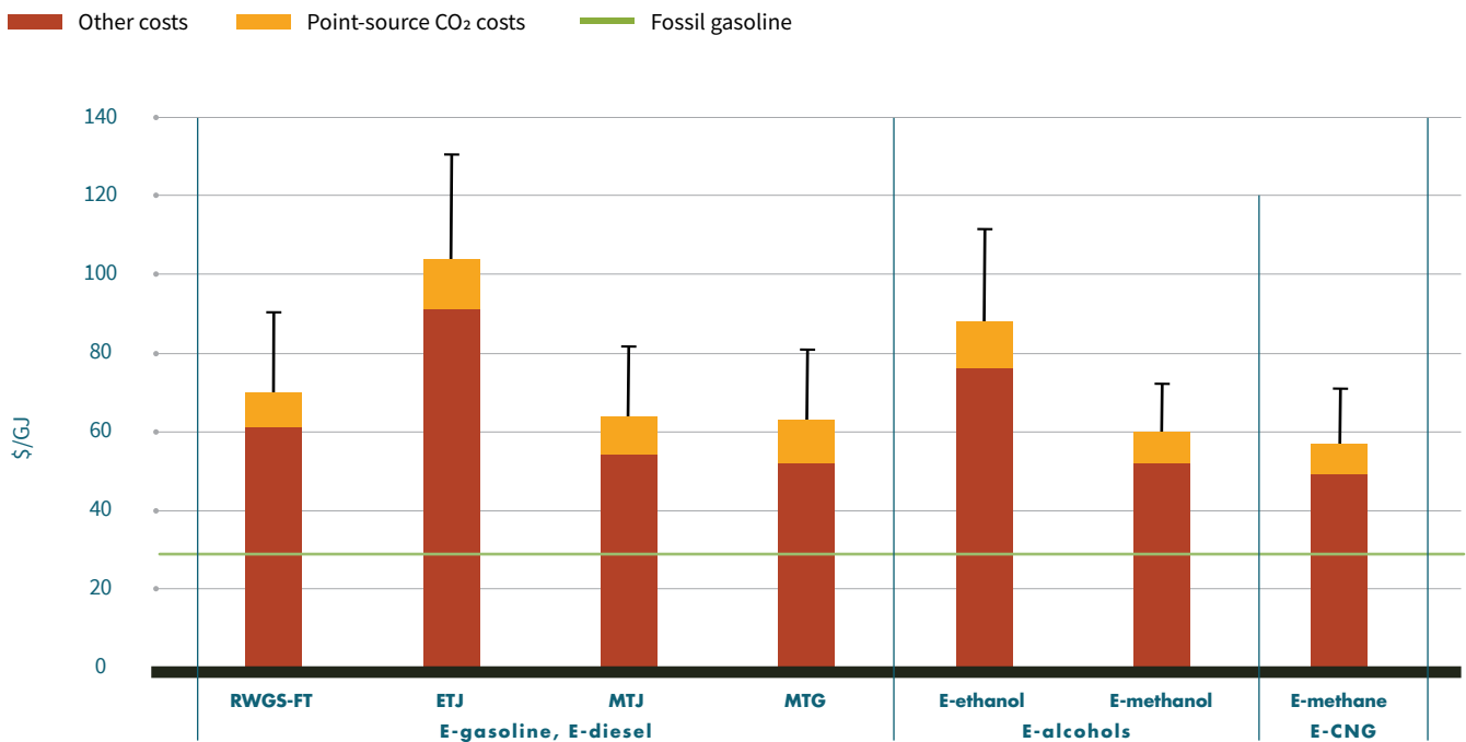
FIGURE 5-5. "FOAK PRODUCTION COST INCREASE WITH USE OF CO 2 FROM DAC
