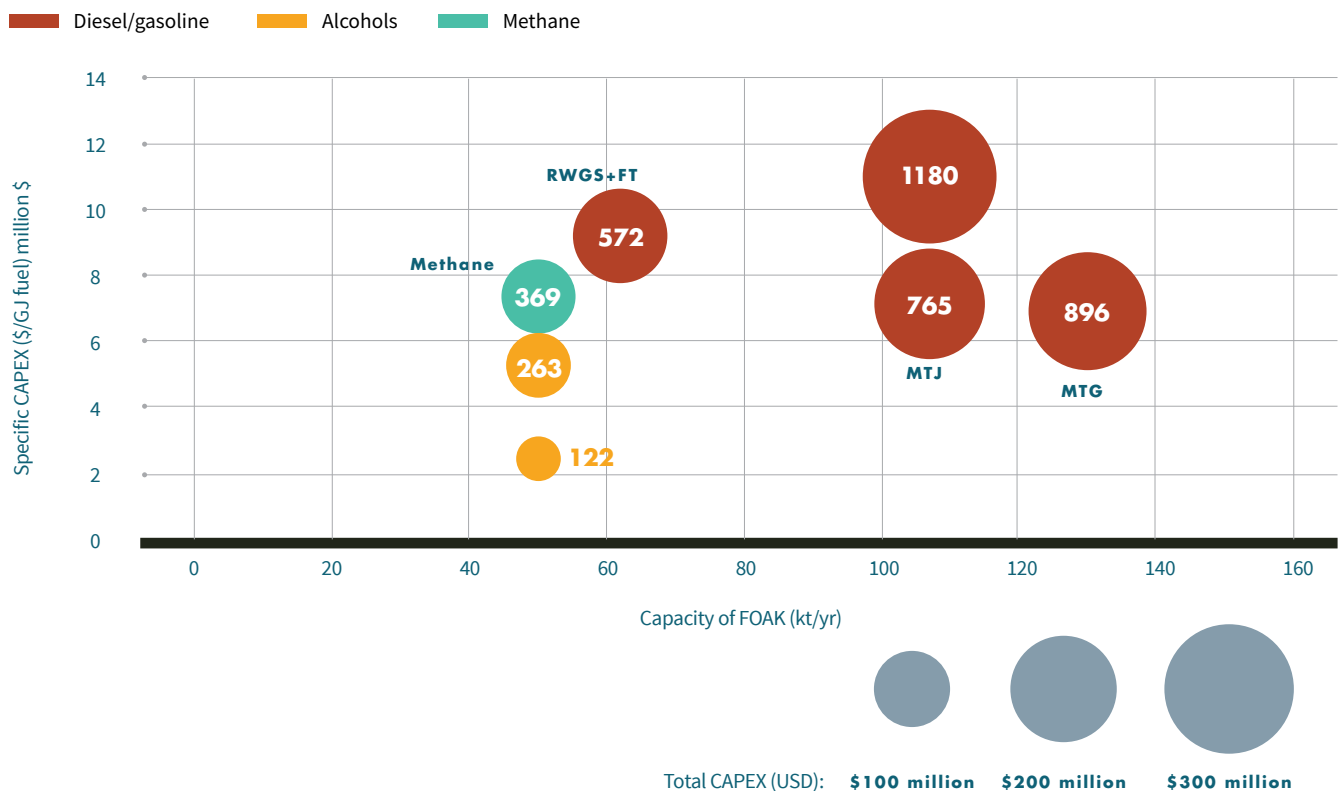
FIGURE 5-8. FOAK CAPACITY AND SPECIFIC CAPEX FOR EACH E-FUEL PATHWAY. (BUBBLE SIZE AND LABEL REPRESENTS TOTAL CAPEX IN $USD MILLIONS).
