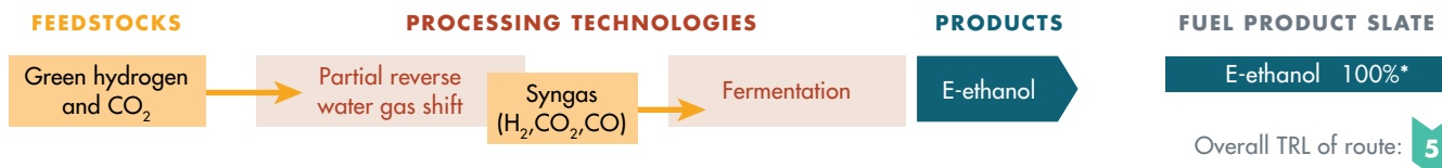
FIGURE 1-5. ETHANOL VIA PRWGS AND FERMENTATION PATHWAY
