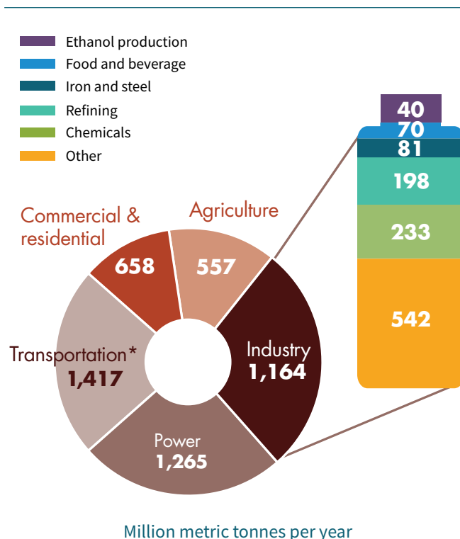
FIGURE 4-6. U.S. CARBON DIOXIDE EMISSIONS BY SECTOR IN 2022.
