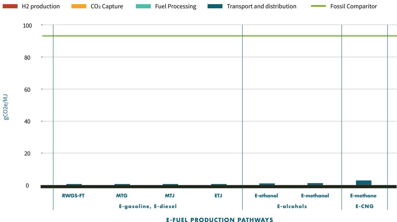
FIGURE 3-4. WELL-TO-WHEEL GHG EMISSIONS FOR E-FUEL PATHWAYS REPRESENTING FUTURE PRODUCTION CONFIGURATIONS.
