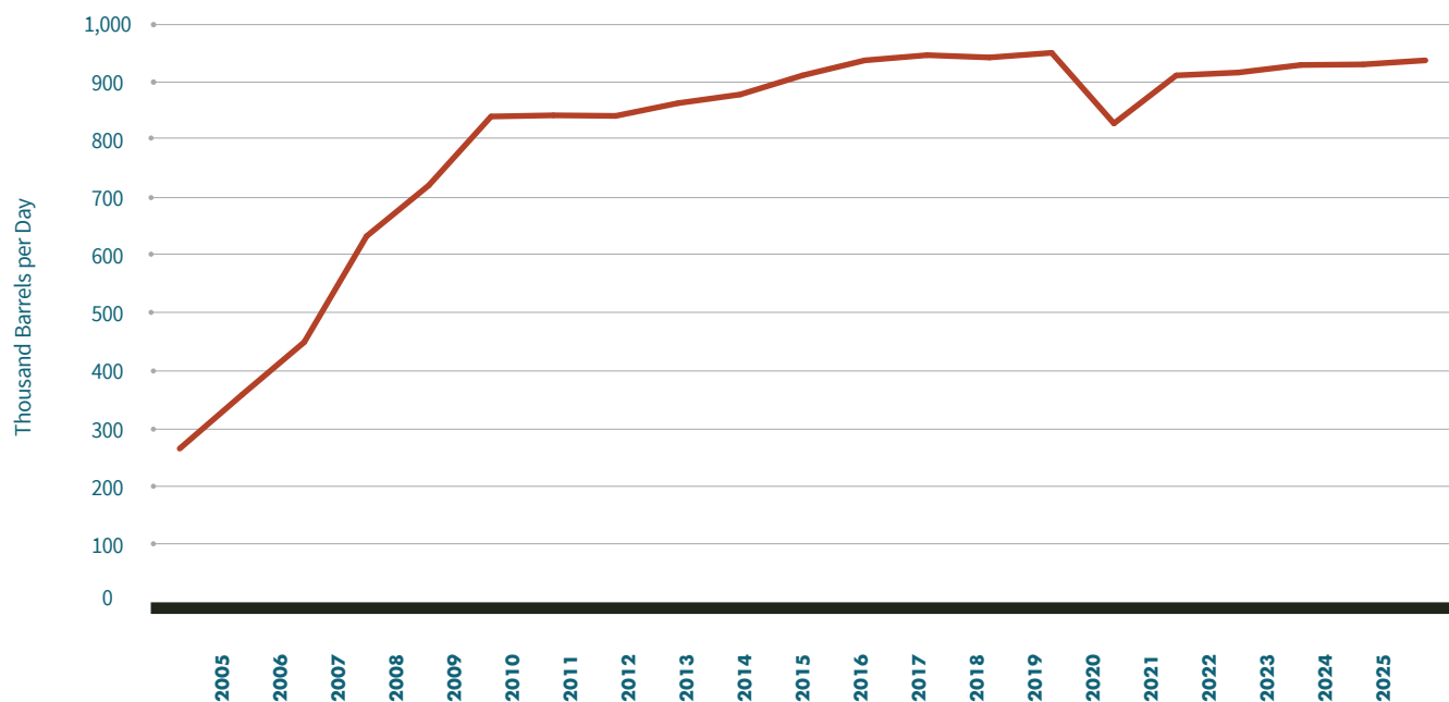
FIGURE 7: ETHANOL CONSUMPTION
